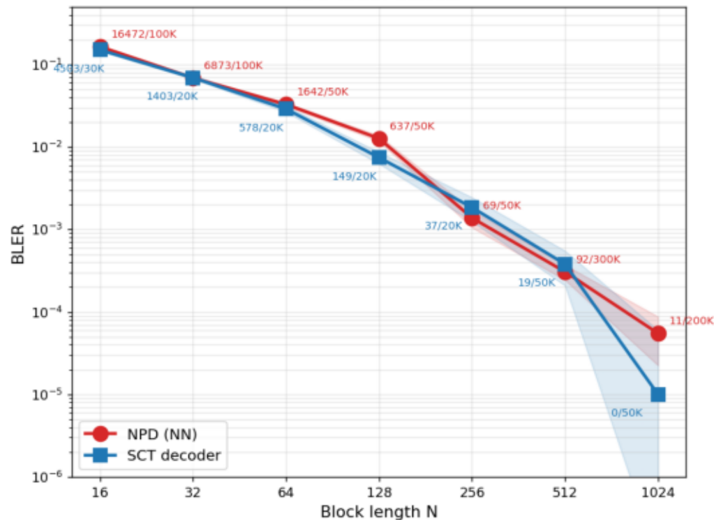
ISI-MAC ( h=0.3 , SNR=6 dB) NPD vs SCT decoder
