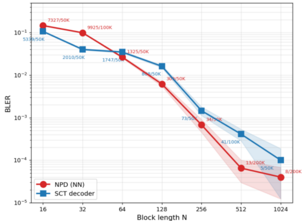
MA-AGN MAC ( \alpha=0.5 , SNR=6 dB) NPD vs SCT decoder
