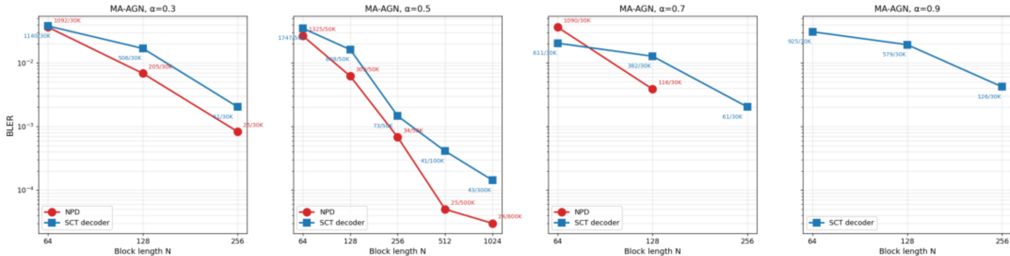
MA-AGN MAC \alpha sweep: NPD vs SCT decoder. SNR=6 dB. Annotations: errs / CW.
