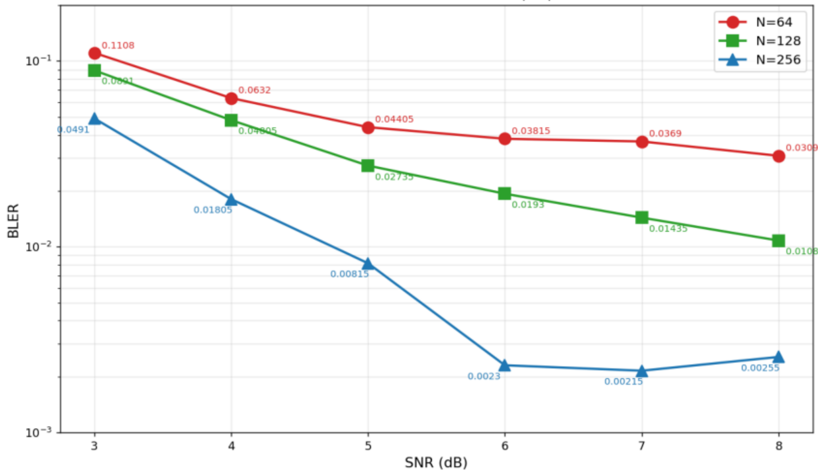
ISI-MAC waterfall: joint trellis SC (own MC at design SNR-3 dB) h=0.3, Class C corner-rate. 20K CW per point.
