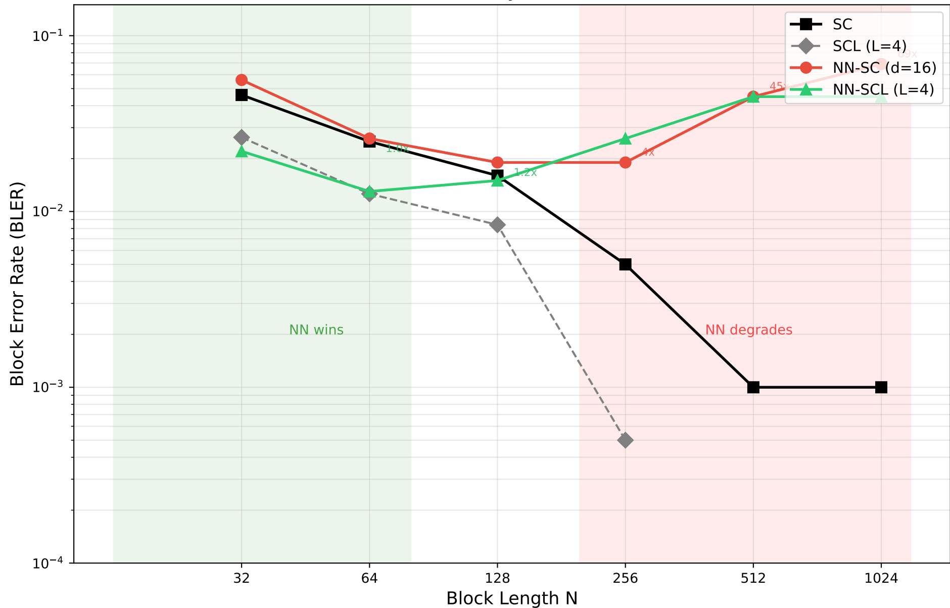
GMAC Class B (SNR=6dB, R_u \approx R_v \approx 0.48 ) Neural vs Analytical Decoders
