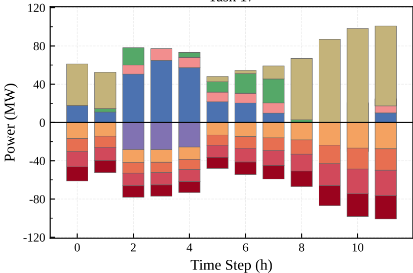
Task 17
