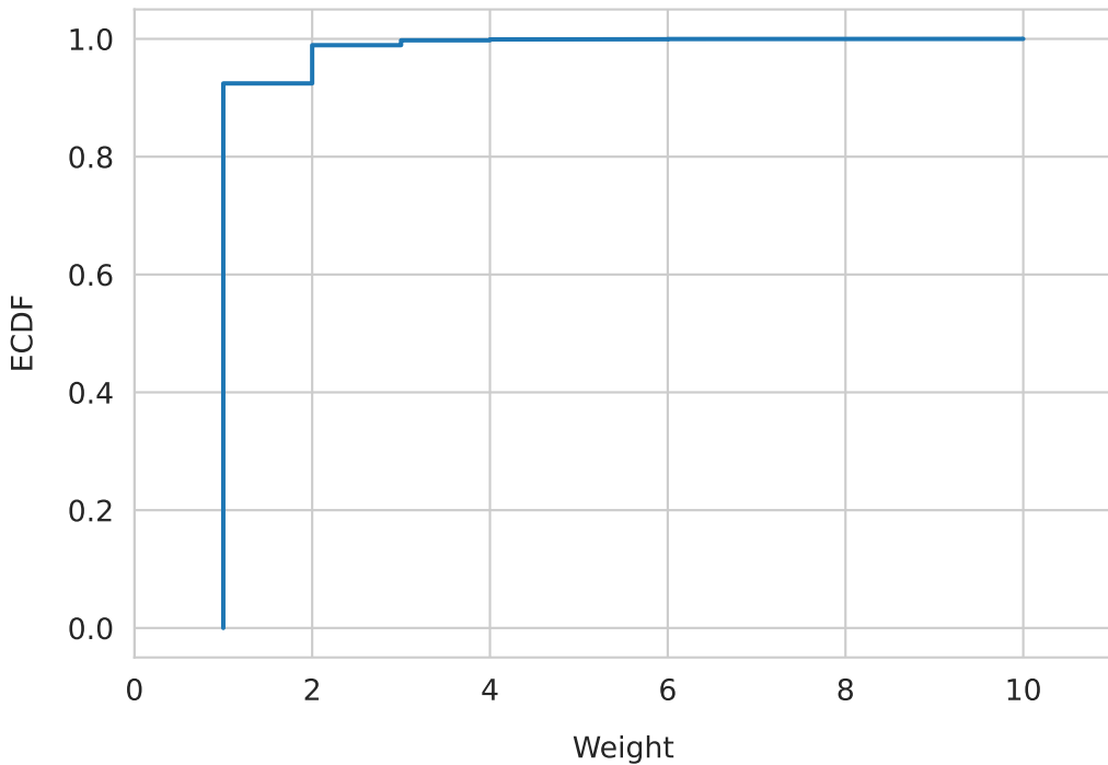
Pairwise KC-KC Claw Connectivity
