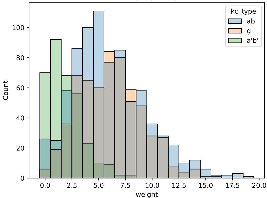
KC->APL non-claw synapses, per KC
