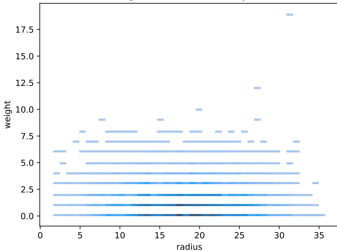
APL->KC claw weight vs radius (from calyx center)
