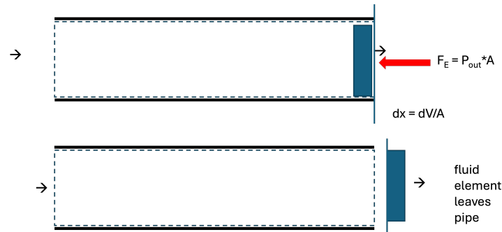
Fig. 7: A “slug” of fluid (the system) pushes out of the pipe.
