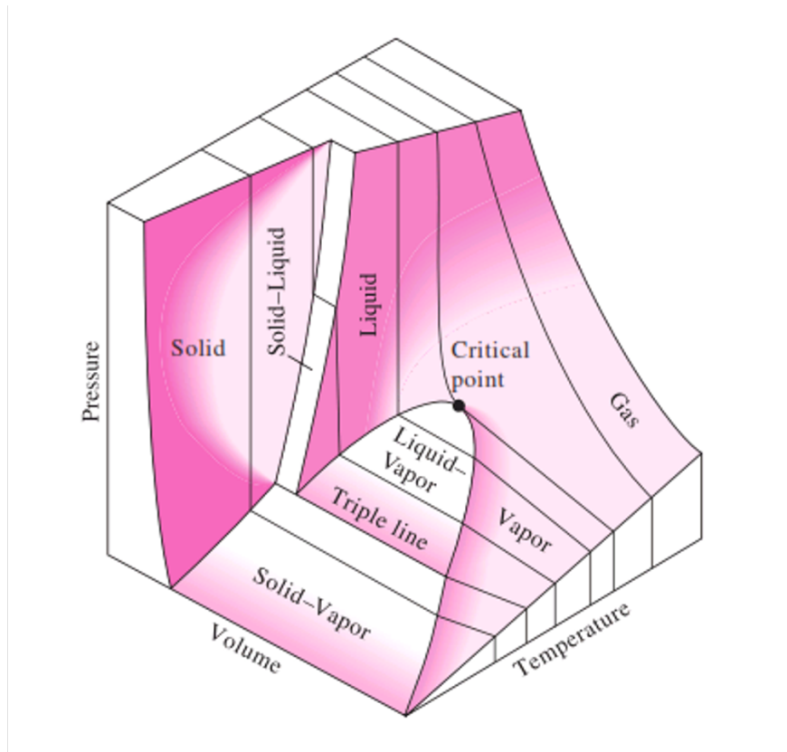
Fig. 8: Schematic 3D P-V-T surface showing solid, liquid, vapor regions, critical point, and a triple line. Image courtesy of Sounak Bhattacharjee.
