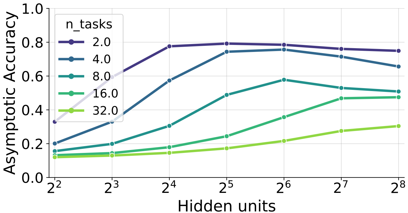
Dense — Asymptotic Accuracy vs Hidden Units (best LR per cell)
