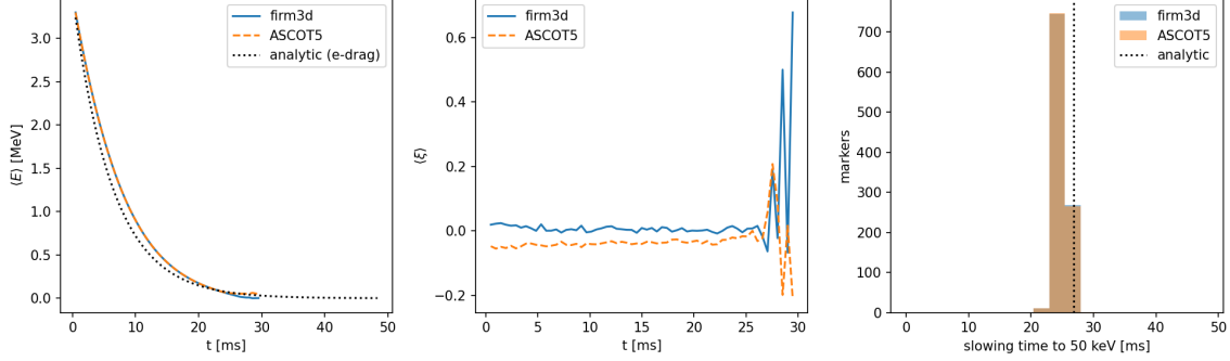
Figure 1: firm3d vs. ASCOT5, uniform 1 keV plasma, N = 1024 : mean energy \langle E(t) \rangle against the analytic electron-drag estimate v = v_0 e^{-t/\tau_{se}} (left); mean pitch \langle \xi(t) \rangle , shown for qualitative comparison only since it is geometry-sensitive (centre); and the distribution of per-particle slowing-down times to 50 keV against the analytic Spitzer estimate (right).
