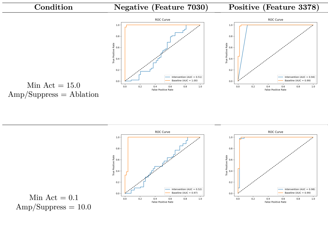
Figure 8 - Area Under the Receiver Operating Characteristic (AUROC) curve for 100 DNA sequences
