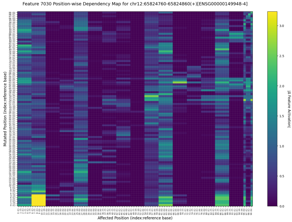
Figure 9 - Dependency Maps showing selected feature sensitivity at a given position (x-axis) for substitution at a selected position (y-axis) in a selected cisplatin-binding sequence. Heat color represents
