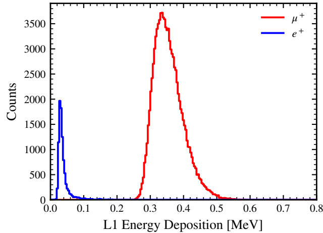
Figure 6: Energy deposit from muons and positrons in the first L1 upstream layer.
