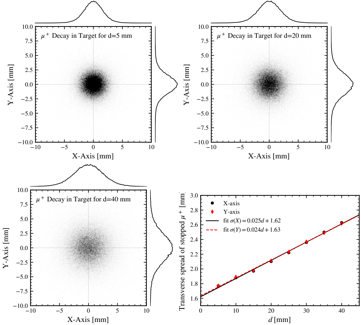
Figure 7: Transverse distribution of stopped muons in the target for selected inner-layer distances d . The lower-right panel shows the standard deviation of the stopped-muon transverse distribution as a function of d . This plot is used as a stopping-distribution sanity check, not as the primary reconstruction residual.
