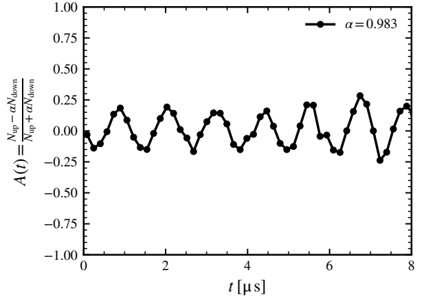
(b) Corresponding upstream-downstream asymmetry.
