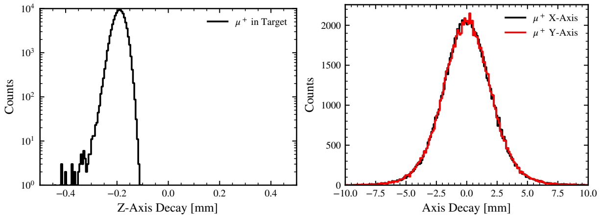
Figure 5: Muon stopping distribution in the aluminium target. Left: longitudinal distribution along z . Right: transverse distributions in x and y .
