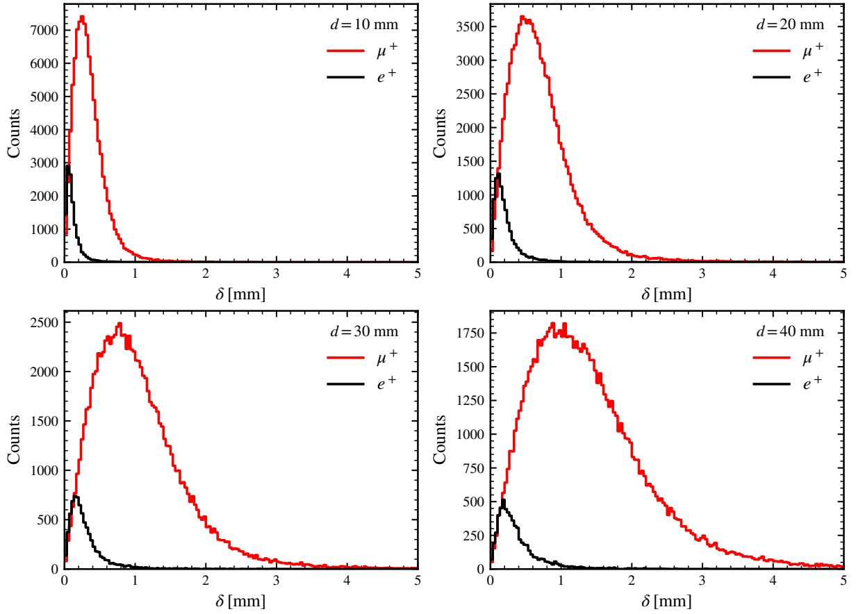
Figure 8: Distribution of \delta_\mu (red) and \delta_e (black) for different distances d .
