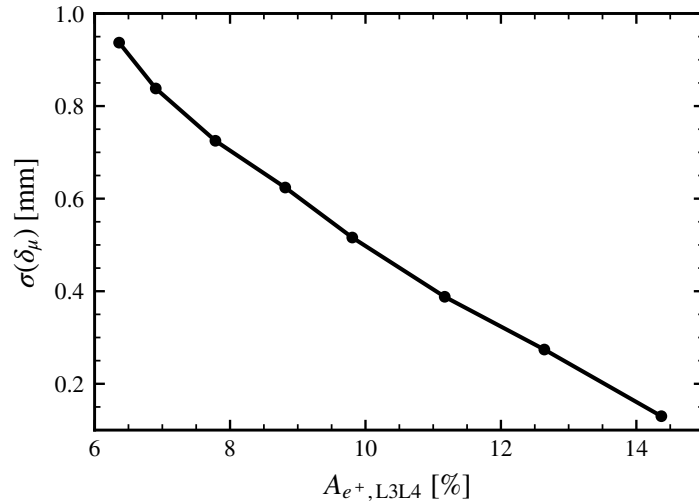
Figure 9: Correlation between the muon reconstruction width \sigma(\delta_\mu) and the downstream positron-track acceptance A_{e^+, L3L4} . Each point corresponds to one inner-layer spacing d . In the simplified geometry studied here, smaller d gives both smaller muon residual width and larger downstream positron-track acceptance.
