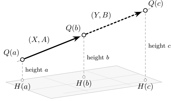
Figure 3: The contradiction setup, with Q(n) = (H(n), n) . The solid arrow labeled (X, A) and the dashed arrow labeled (Y, B) are the directed adjacent displacements. The dotted guide through Q(a), Q(b), Q(c) marks the temporary collinearity assumption.
