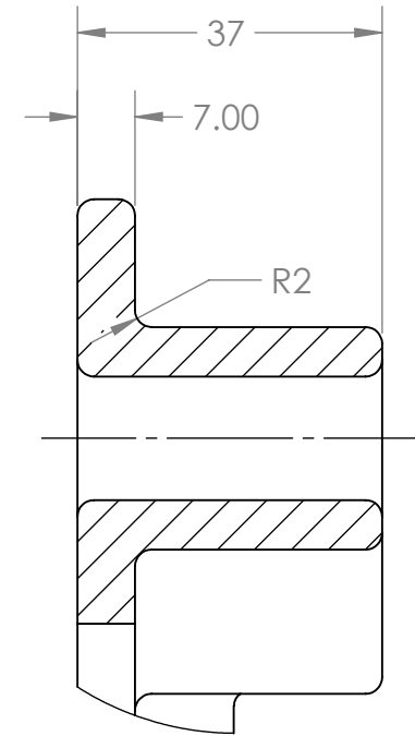
DETAIL B SCALE 1 : 1
