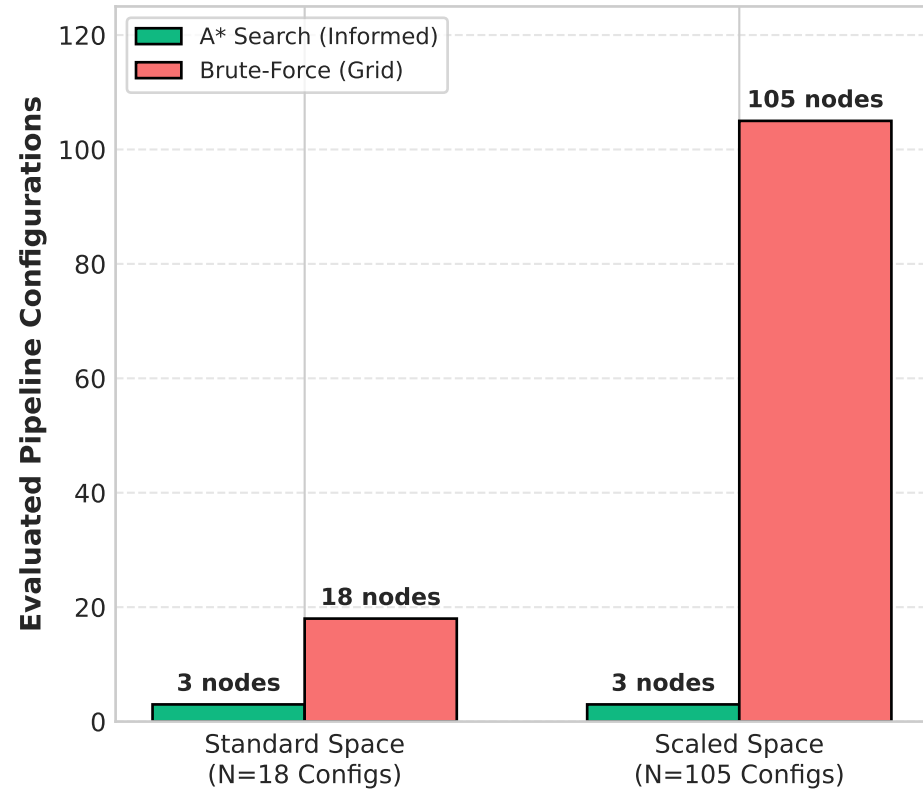
(a) Search Space Evaluations (83.3% / 97.1% Space Pruned)
