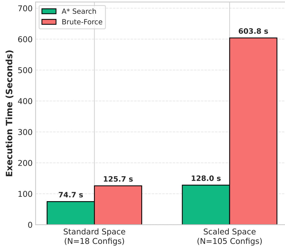
(b) Wall-Clock Computation Time (40.5% / 78.8% Faster)
