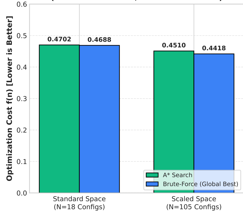
(c) Objective Function Cost f(n) (0.4702 vs 0.4688 / 0.4510 vs 0.4418)
