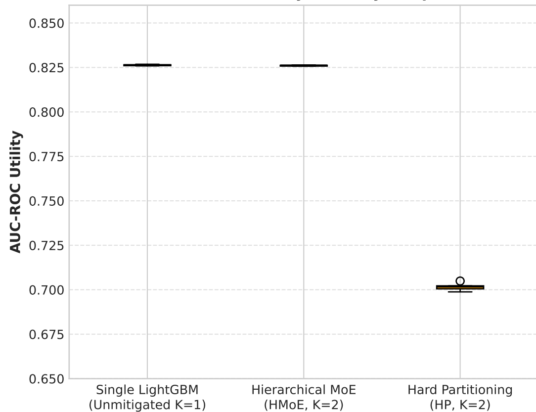
(a) AUC-ROC Utility Stability (5 Splits)
