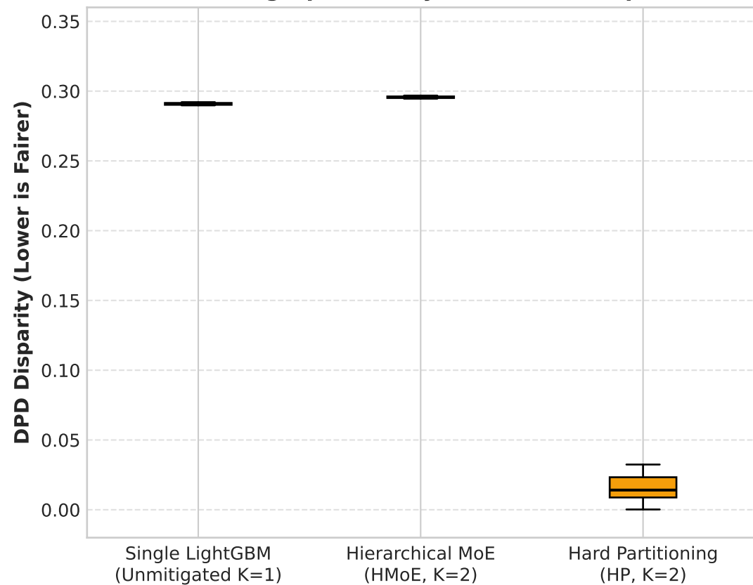
(b) Demographic Parity Difference (5 Splits)
