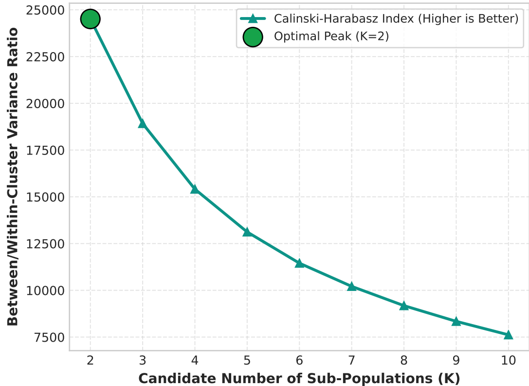
(b) Variance Ratio Criterion across K \in [2, 10]
