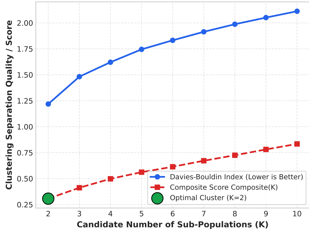
(a) Objective Minimization across K \in [2, 10]
