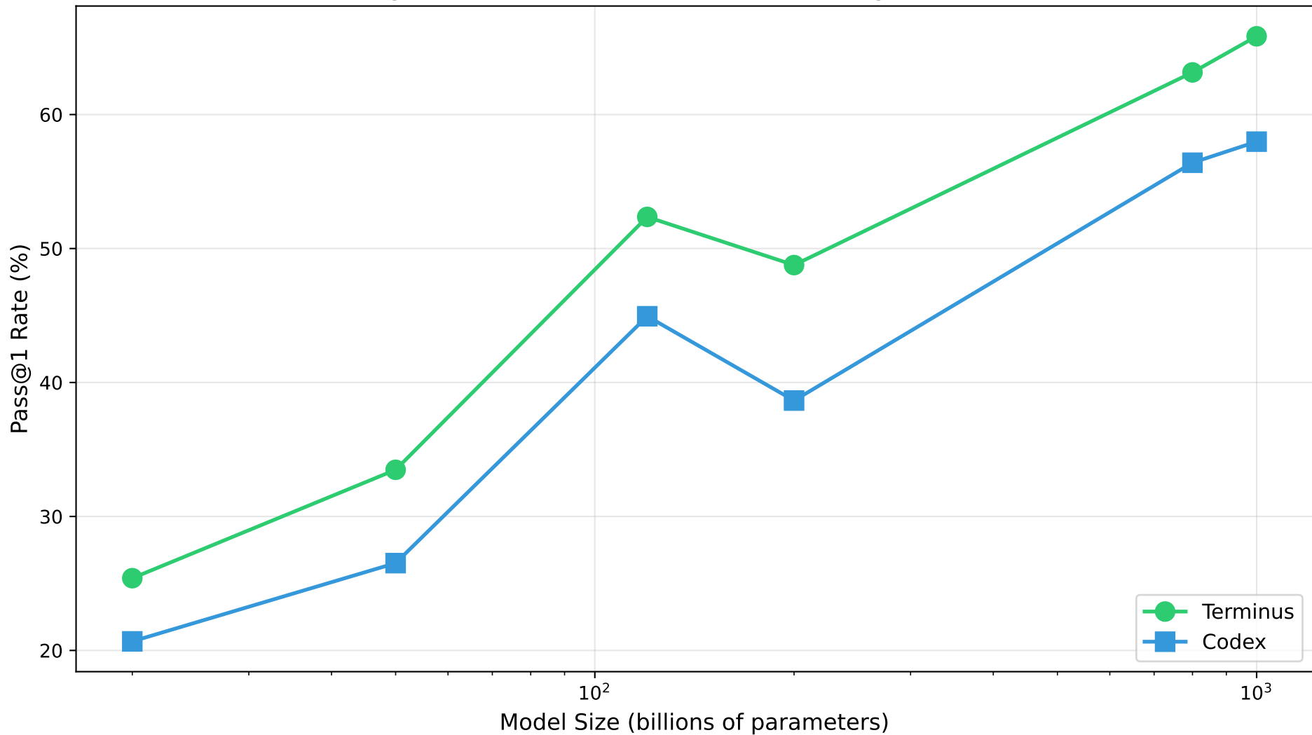
Fig 2a: Pass Rate vs Model Size (Scaling Behavior)
