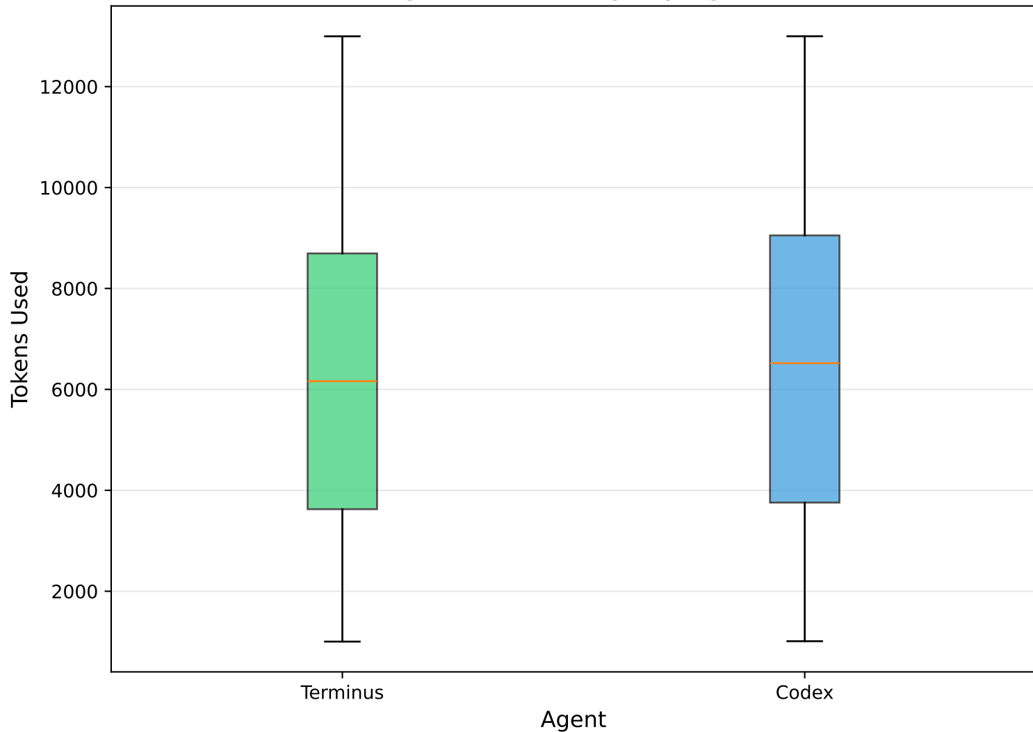
Fig 4b: Token Usage by Agent
