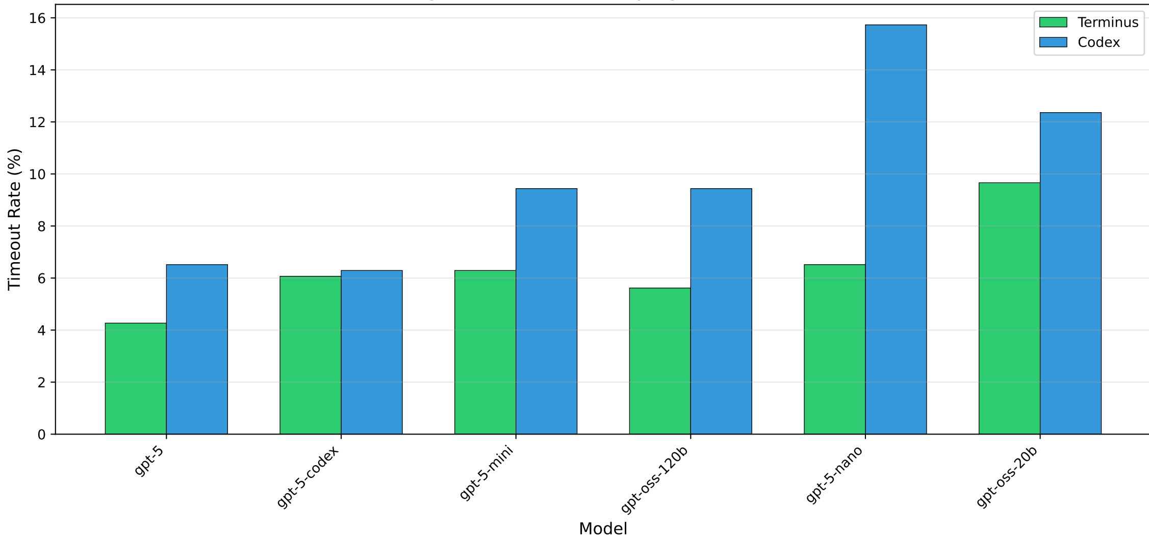
Fig 5b: Timeout Rates by Agent x Model
