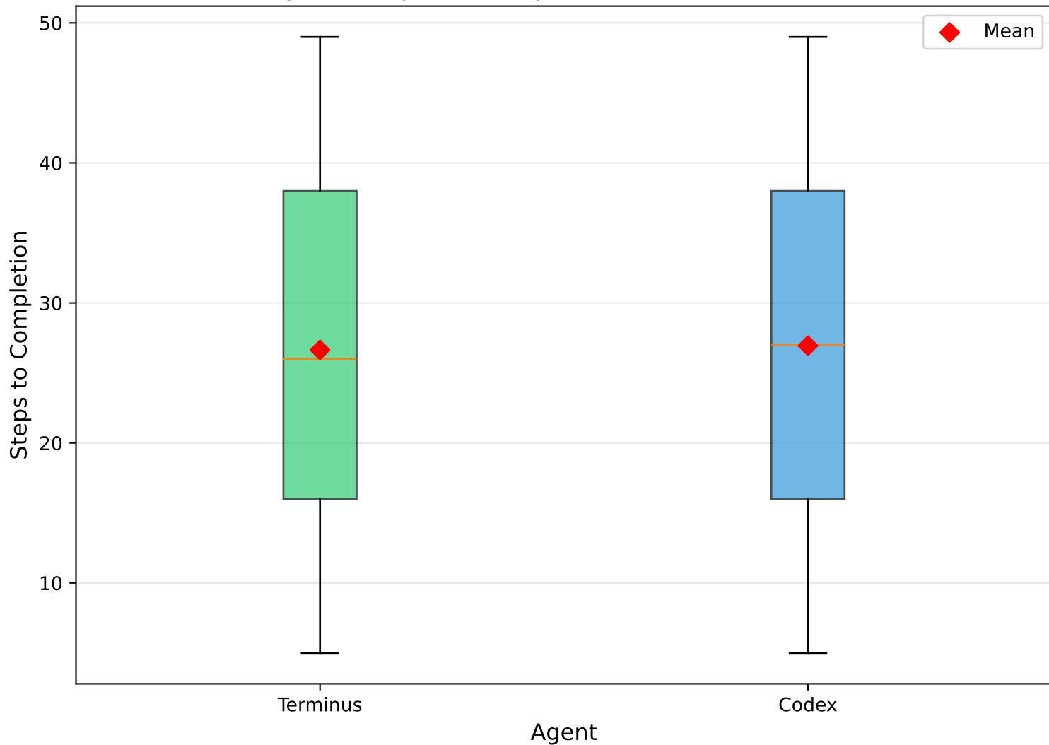
Fig 4a: Steps to Completion (Successful Runs)
