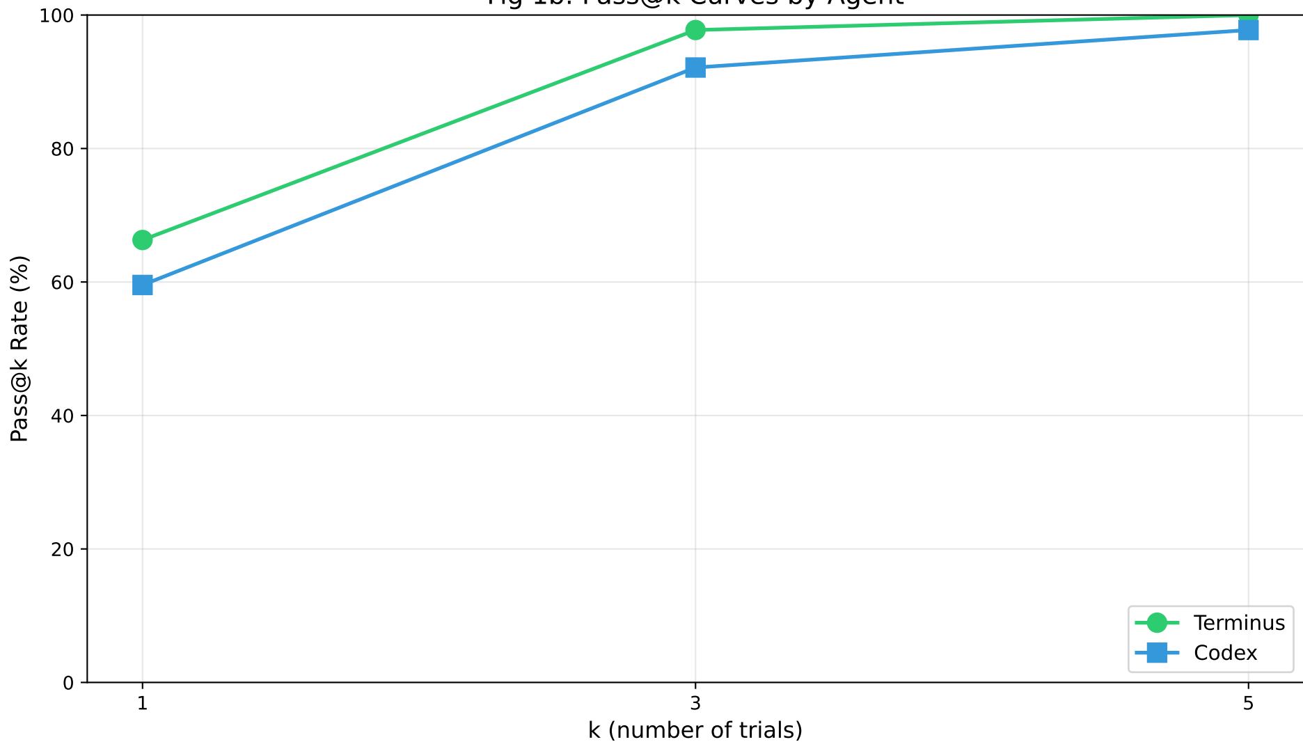
Fig 1b: Pass@k Curves by Agent
