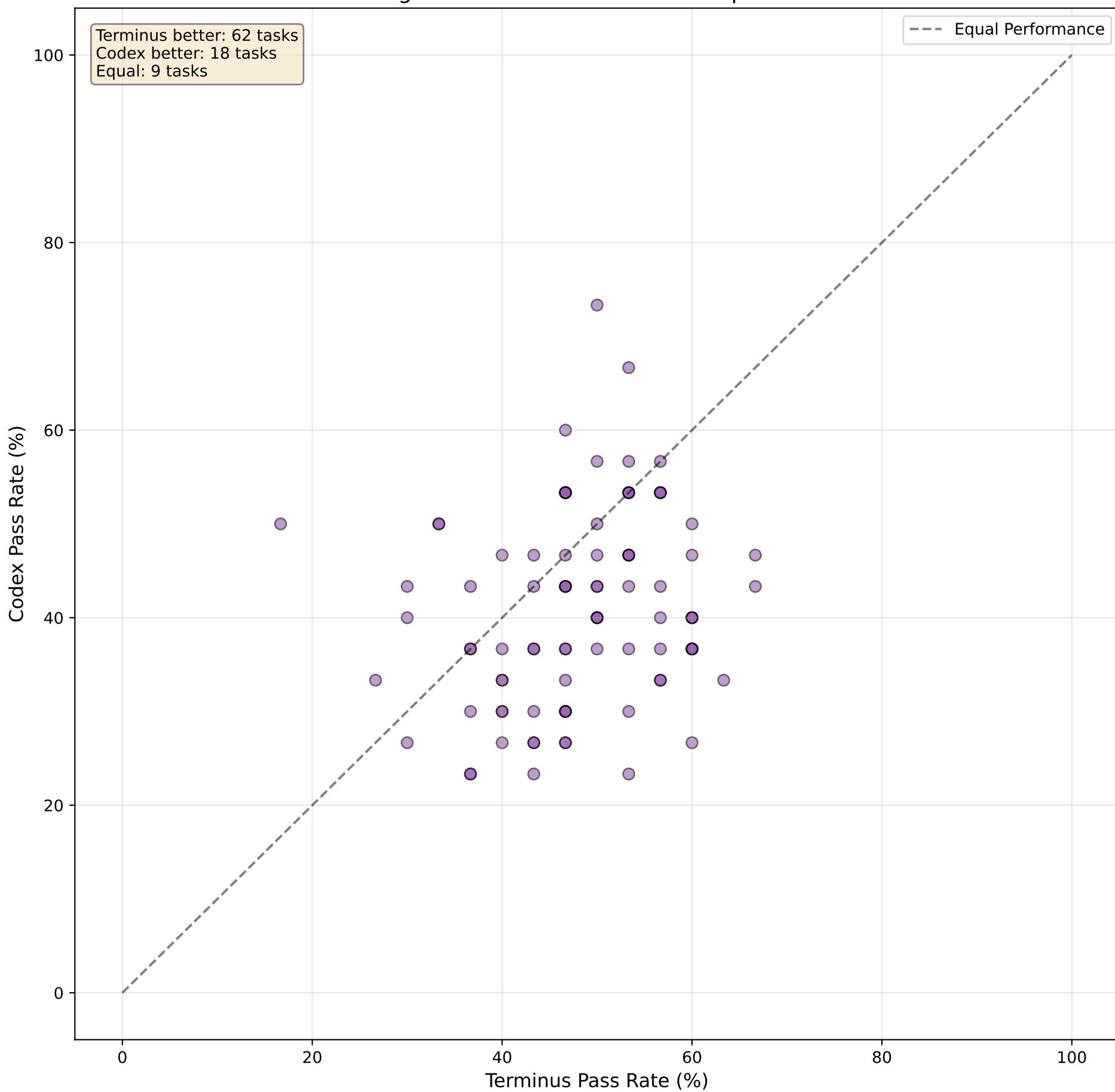
Fig 6b: Head-to-Head Task Comparison
