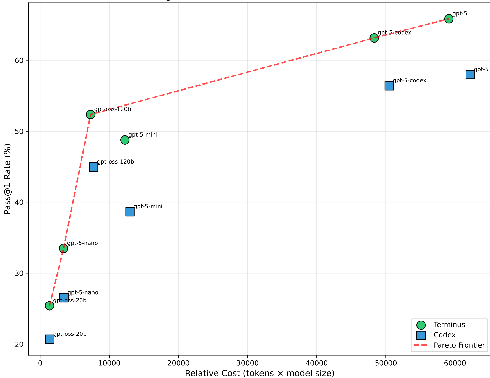
Fig 4c: Pass Rate vs Cost (Pareto Frontier)
