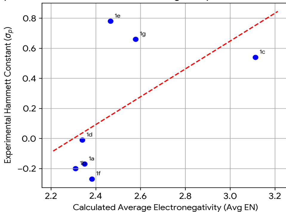
Physical Validation Matrix: Electronegativity vs. Hammett Parameter
