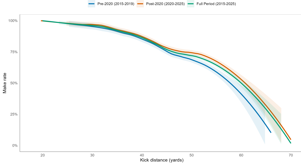
Figure 14: Make rate by kick distance, pre-2020 versus post-2020.
