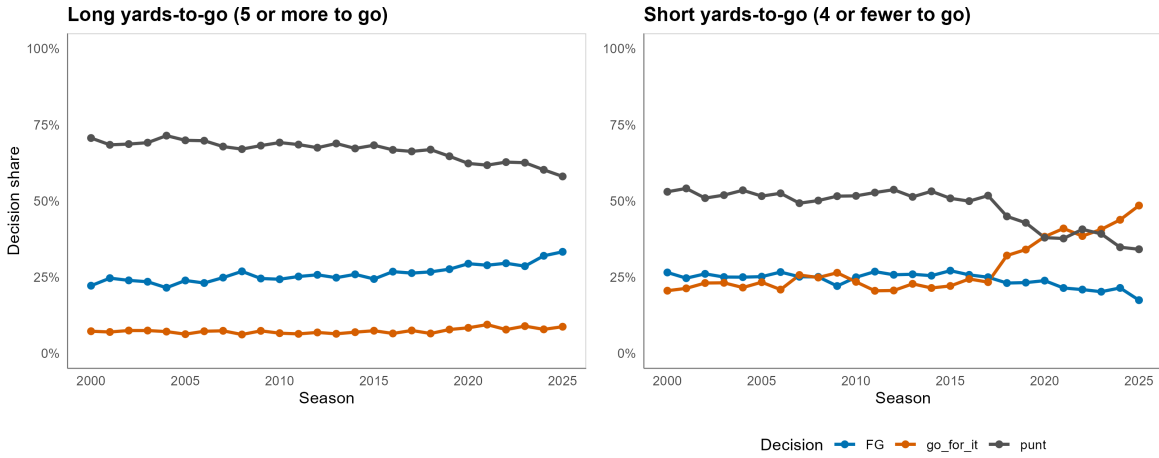
Figure 15: Evolution of fourth-down decision shares by season, split by yards-to-go regime.
