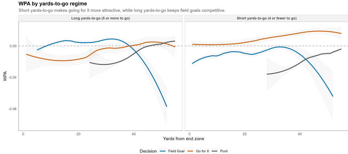
Figure 19: Average win probability added by decision type and field position, split by yards-to-go regime.
