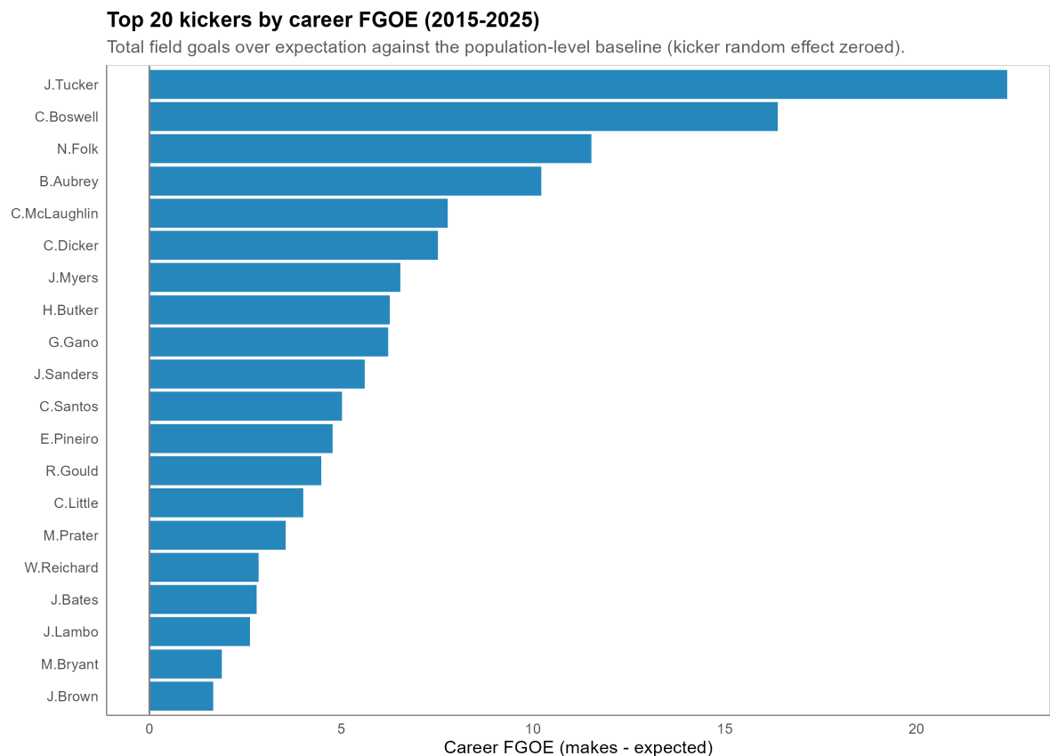
Figure 8: Career FGOE leaderboard, ranked by cumulative FGOE.
