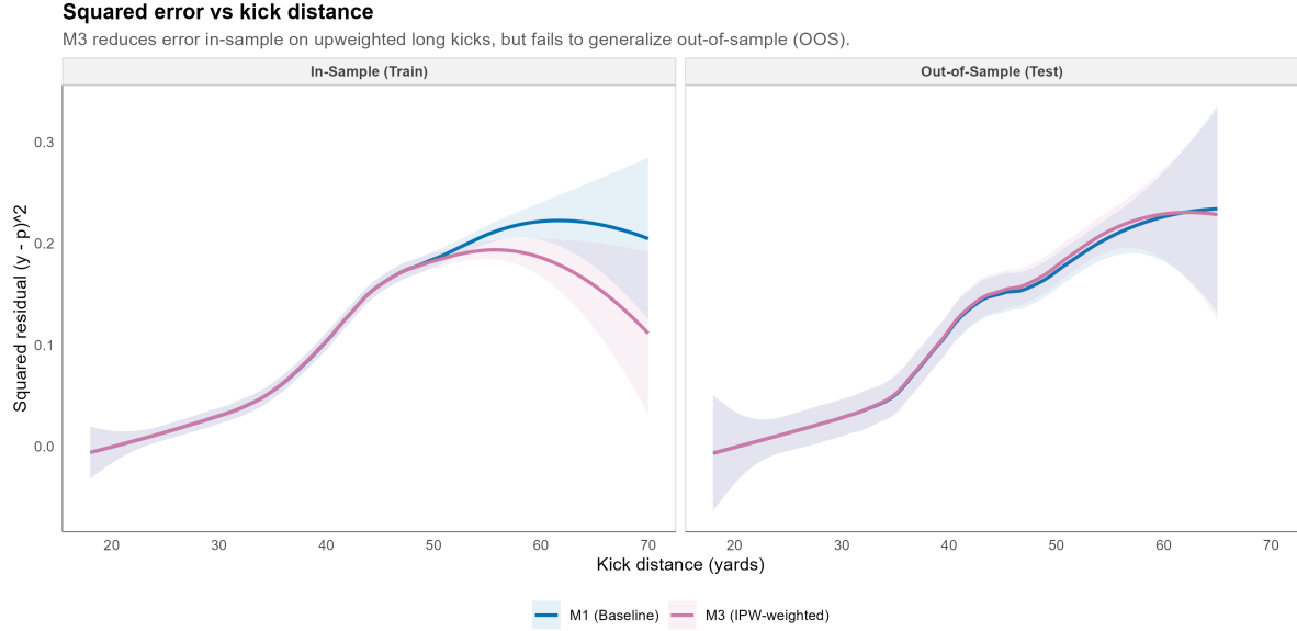
Figure 7: LOESS-smoothed squared error by kick distance, in-sample and out-of-sample.
