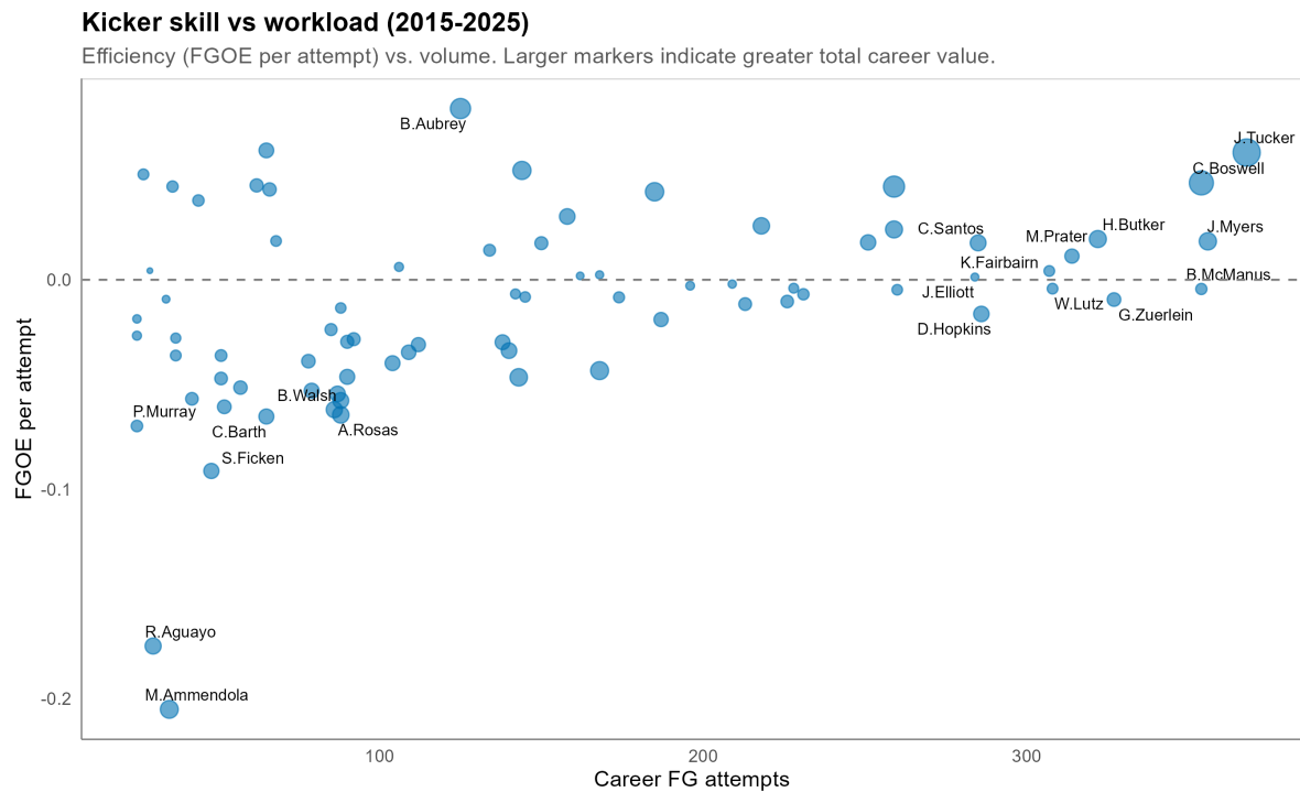
Figure 10: Career FGOE against attempt volume.
