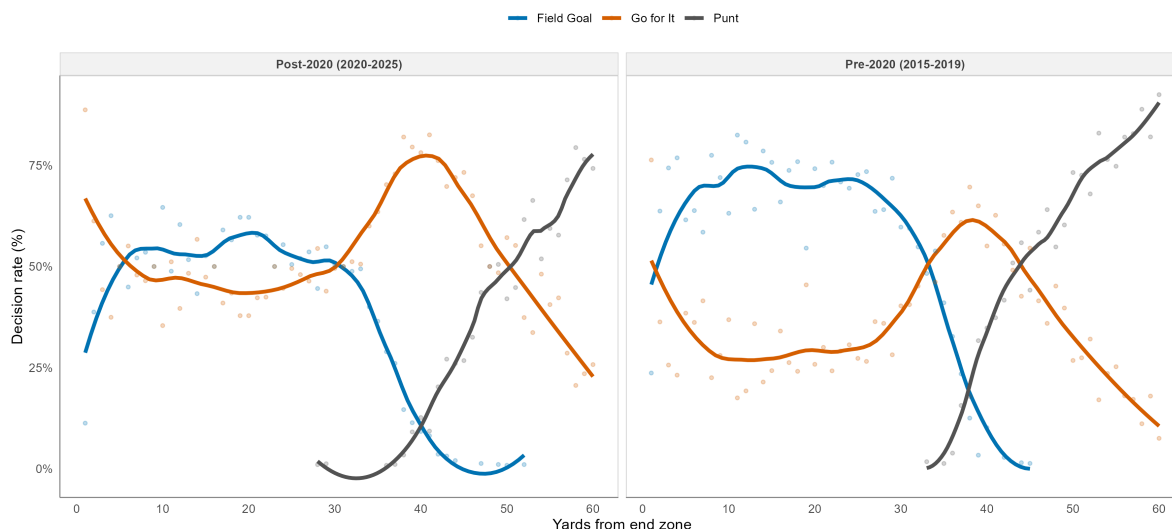
Figure 17: Fourth-down decision shares on short yards-to-go by field position, pre-2020 versus post-2020.
