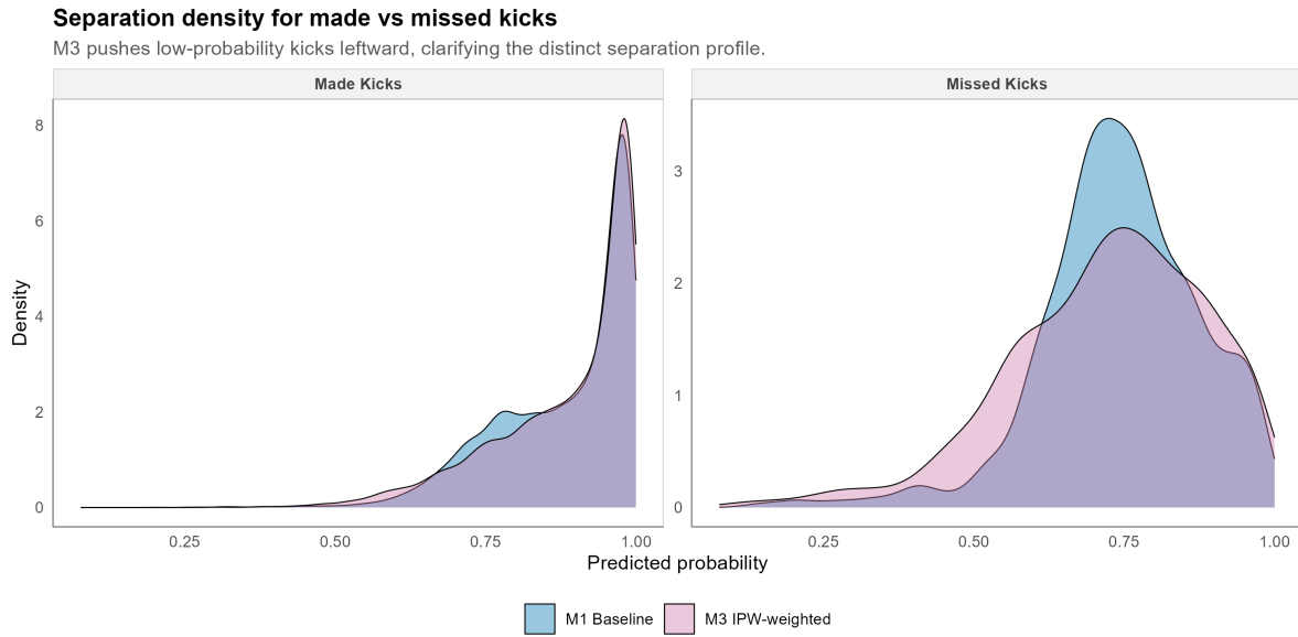
Figure 6: In-sample distribution of predicted make probability, separated by realized outcome.
