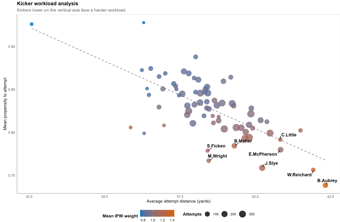
Figure 11: Mean attempt distance against mean attempt propensity, by kicker.
