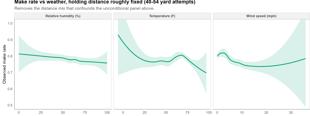
Figure 2: Raw make rate versus each weather covariate within a fixed 40-54 yard distance band.
