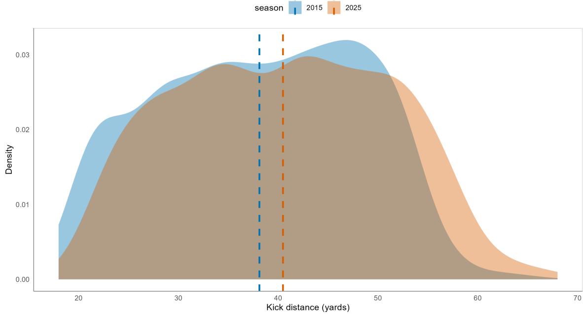
Figure 13: Distribution of field goal attempt distance, 2015 versus 2025.
