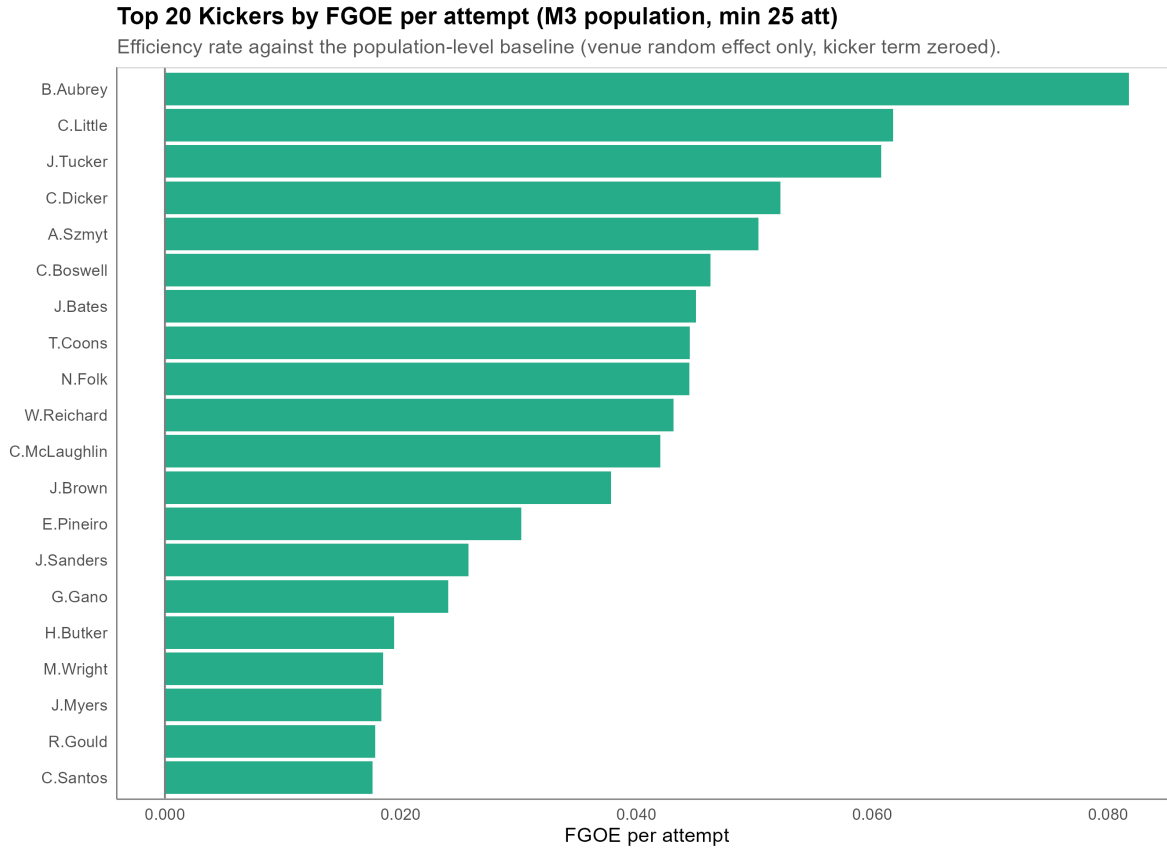
Figure 9: Career FGOE leaderboard, ranked by FGOE per attempt.
