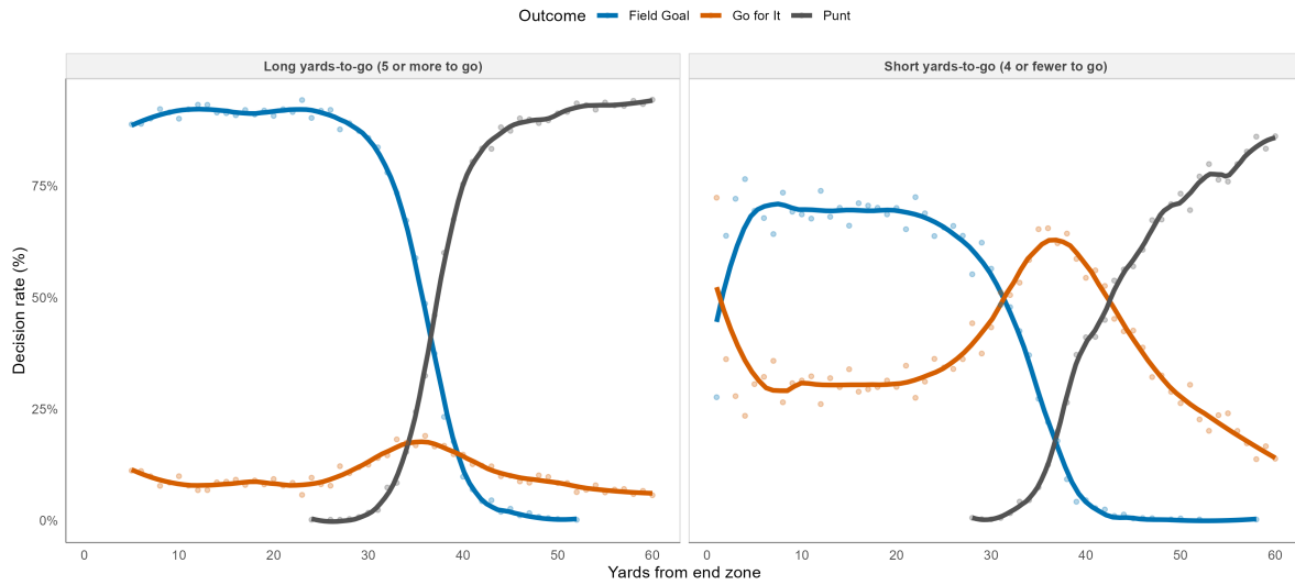
Figure 16: Fourth-down decision shares by field position, split by yards-to-go regime.
