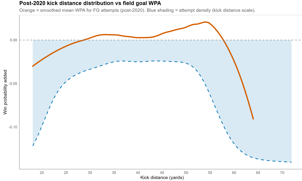
Figure 20: Post-2020 field goal attempt density overlaid on the field goal WPA curve.
