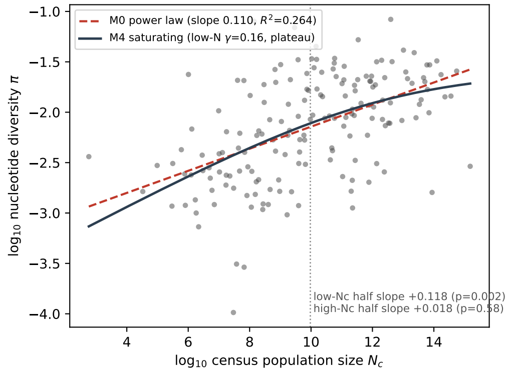
Buffalo's 172 metazoans: rising then plateau
