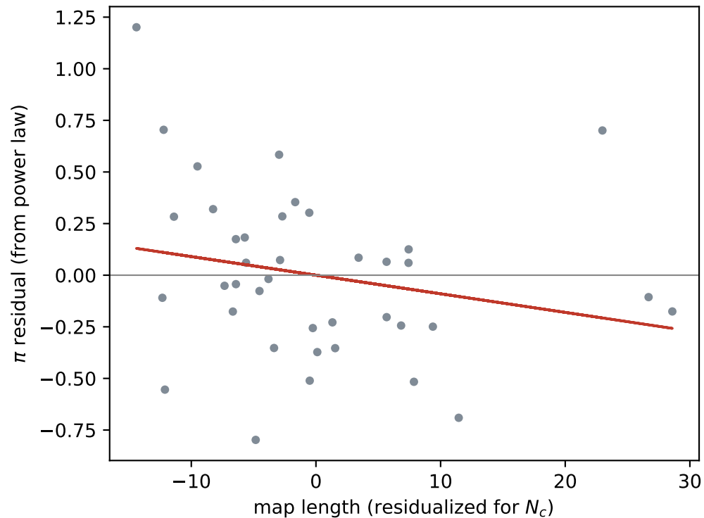
Recombination sign test (n=39): gBGC predicts -, BGS predicts + partial r = -0.22 ( p=0.17 )
