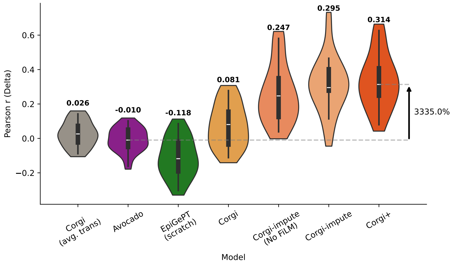
Channel: dnase - Delta over Mean Baseline
