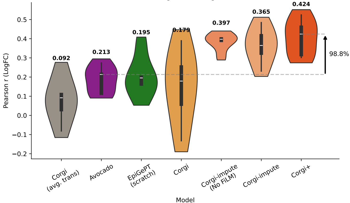
Channel: h3k79me2 - Log Fold Change over Mean Baseline
