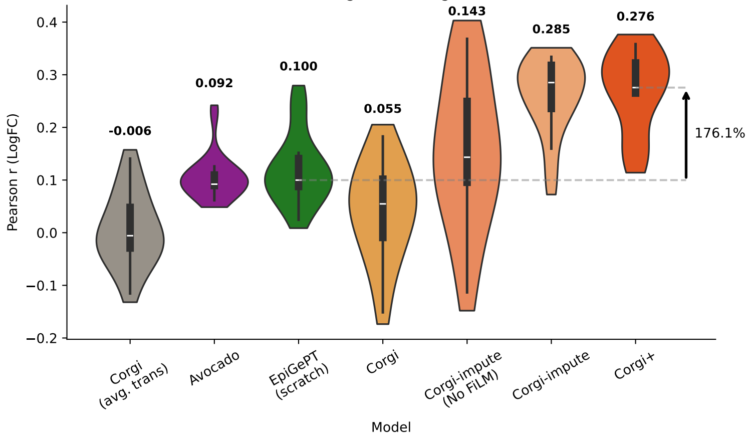
Channel: h3k4me3 - Log Fold Change over Mean Baseline
