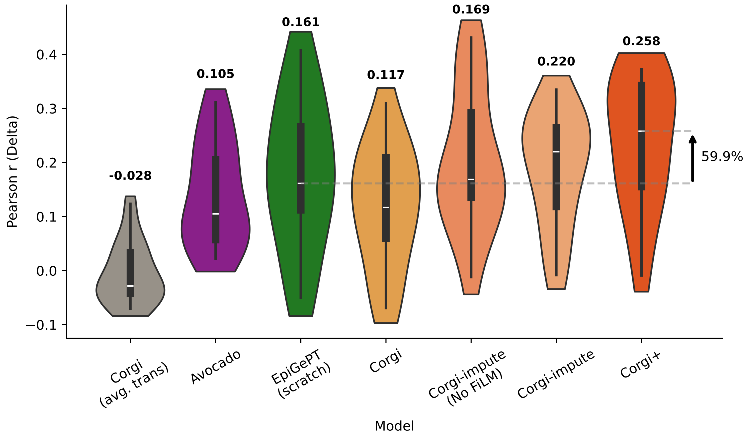
Channel: h3k4me1 - Delta over Mean Baseline
