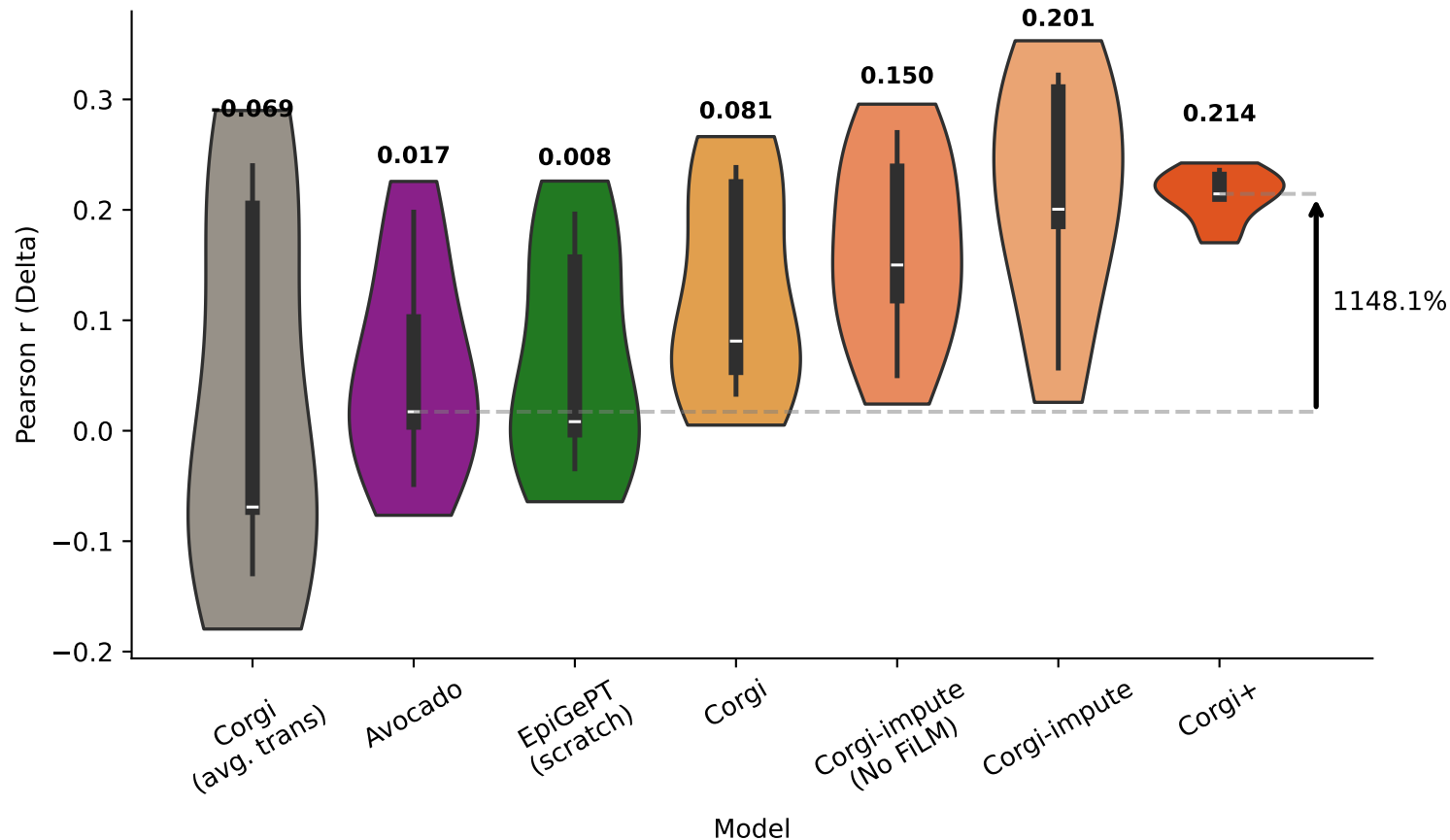
Channel: atac - Delta over Mean Baseline
