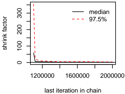
prior
