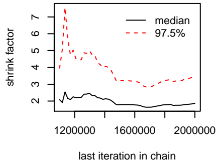
likelihood
