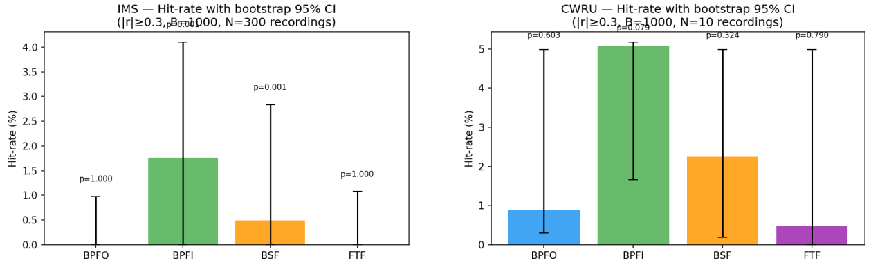
Figure 3. Per-BPFx hit-rate (% , |r| \geq 0.30 ) with bootstrap 95 % CI for the Mamba-xLSTM-Net backbone on the two diagnostic-style datasets. Left: IMS (BPFI 1.76 % and BSF 0.49 % with p = 0.001 ). Right: CWRU (BPFI 5.08 % as the dominant frequency; wide CIs reflect the small recording pool and the permutation p -values do not pass the 0.05 threshold).
