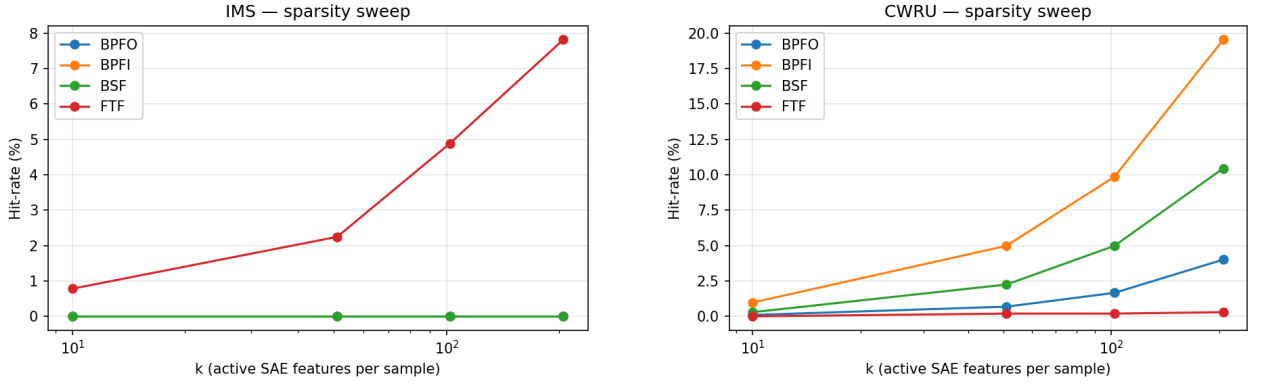
Figure 9. Sparsity sweep on the diagnostic-style datasets. Left: IMS — only FTF rises monotonically; BPFO, BPFI, and BSF stay at zero across all k . Right: CWRU — BPFI grows from 0.98% at k = 10 to 19.53% at k = 205 and dominates the four BPFx; BSF tracks BPFI with about half the magnitude. The CWRU sweep shows the steepest growth of any dataset, reflecting the discrete severity-label structure of the target.
