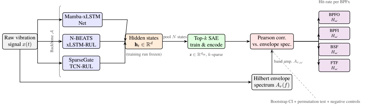
Figure 1. Conceptual overview of the proposed mechanistic interpretability pipeline. Raw vibration signals pass through one of three frozen backbone RUL models to produce hidden-state pools \mathbf{h}_t . A Top- k Sparse Autoencoder (SAE) is trained post-hoc on those states and produces sparse latent codes \mathbf{z} . Pearson correlations between SAE feature activation profiles and Hilbert envelope-spectrum amplitudes at the four bearing characteristic frequencies yield per-BPFx hit-rates H_\omega , evaluated with bootstrap 95 % confidence intervals, permutation tests, and two negative controls.
