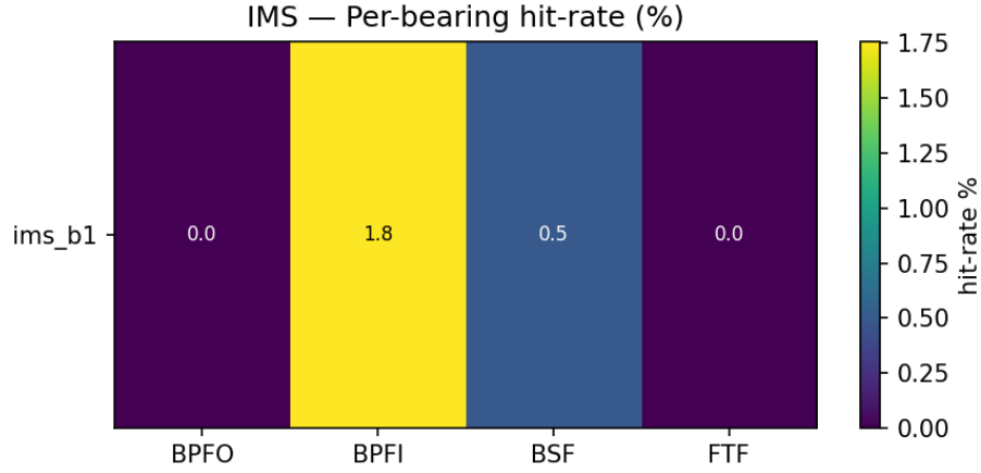
Figure 5. Per-bearing BPFx hit-rate (%) for the Mamba-xLSTM-Net backbone on the IMS dataset (single-row by design — only the acoustically dominant channel ims_b1 is scanned). The corresponding CWRU breakdown is omitted because each CWRU file is below the five-recording threshold of the bearing-stratified estimator; pooled CWRU values are reported in Table 5 and per-architecture values in Table 8.
