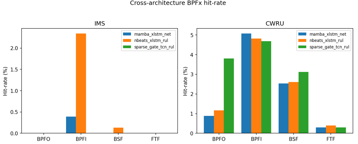
Figure 6. Cross-architecture BPFx hit-rate (%) for all three backbone architectures (fresh SAE per architecture, k = 51 , threshold |r| \geq 0.30 ) on the four benchmark datasets. Mamba-xLSTM-Net leads on PHM2012; on XJTU-SY all three architectures show non-zero hit-rates across multiple BPFx; IMS hit-rates are uniformly low; on CWRU the three architectures converge to a BPFi-dominant profile regardless of inductive bias.
