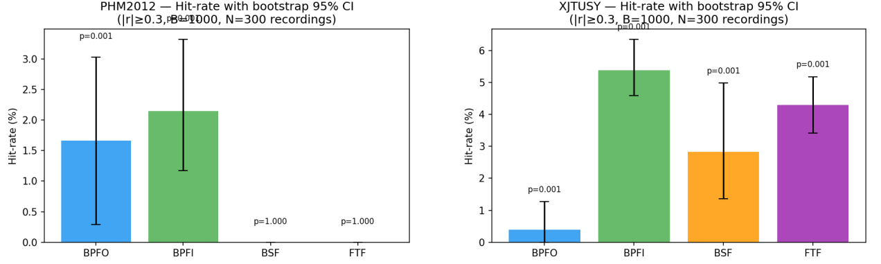
Figure 2. Per-BPFx hit-rate (% , |r| \geq 0.30 ) with bootstrap 95 % CI for the Mamba-xLSTM-Net backbone on the two RUL benchmarks under the journal-extension protocol. Left: PHM2012 (BPFI/BPFO dominant; BSF/FTF zero). Right: XJTU-SY — the bootstrapped re-run shows non-zero contributions on multiple BPFx, but the dissertation analysis with a longer SAE training budget (Table 5) recovers the expected outer-race-dominant profile (B. Wang et al., 2020); the dissertation point estimate (BPFO 2.2 %) lies within the CI shown here. Error bars are the 95 % CI from B = 1,000 bootstrap resamples of the recording pool; annotations report the one-sided greater permutation p -value.
