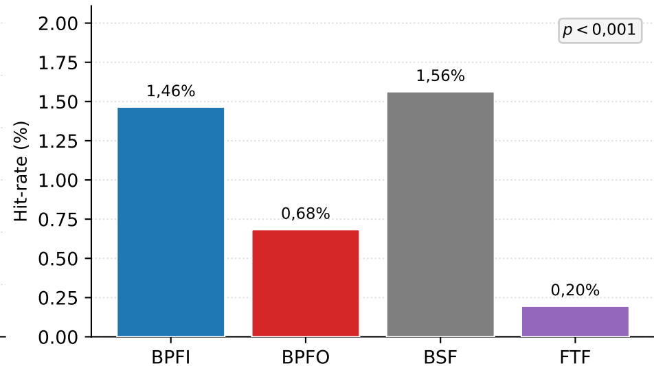
CWRU — underpowered
