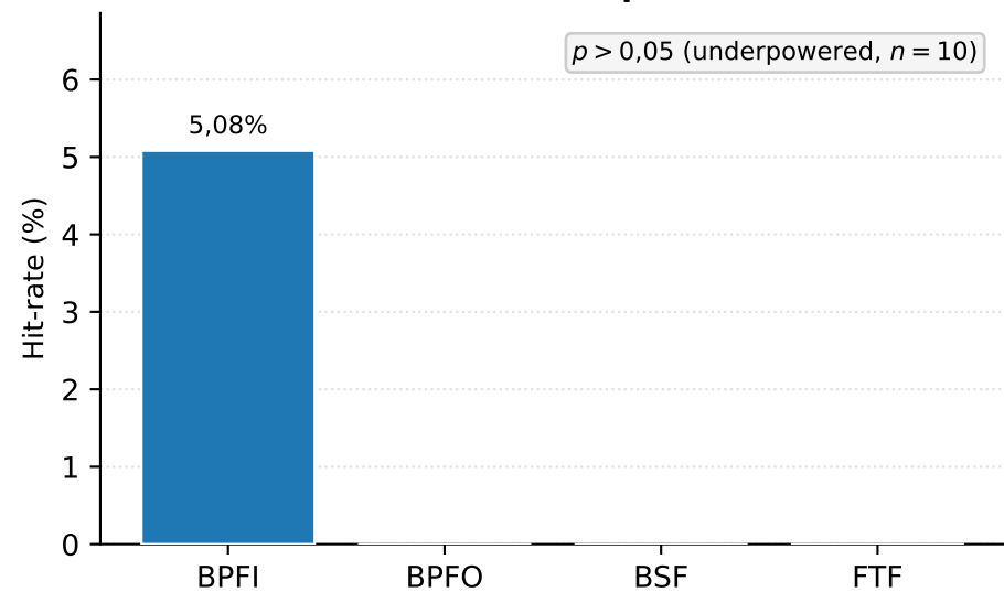
CWRU — underpowered
