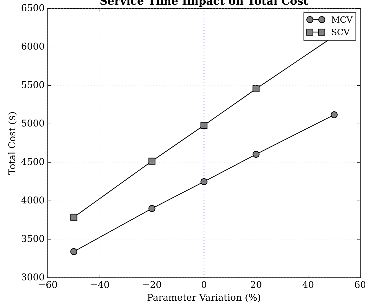
Service Time Impact on Total Cost
