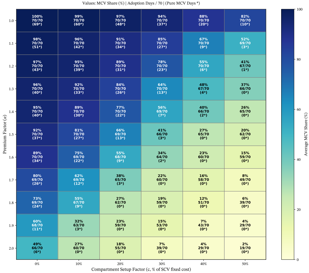
Figure 4: Effect of premium factor ( \alpha ) and compartment setup factor ( c ) on fleet composition.
