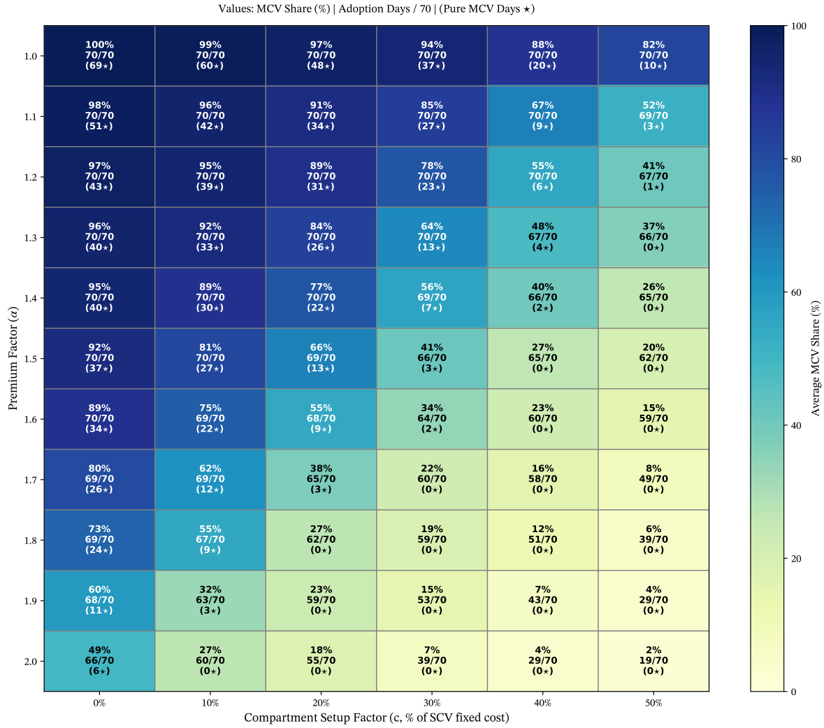
Figure 4: Effect of premium factor ( \alpha ) and compartment setup factor ( c ) on fleet composition.
