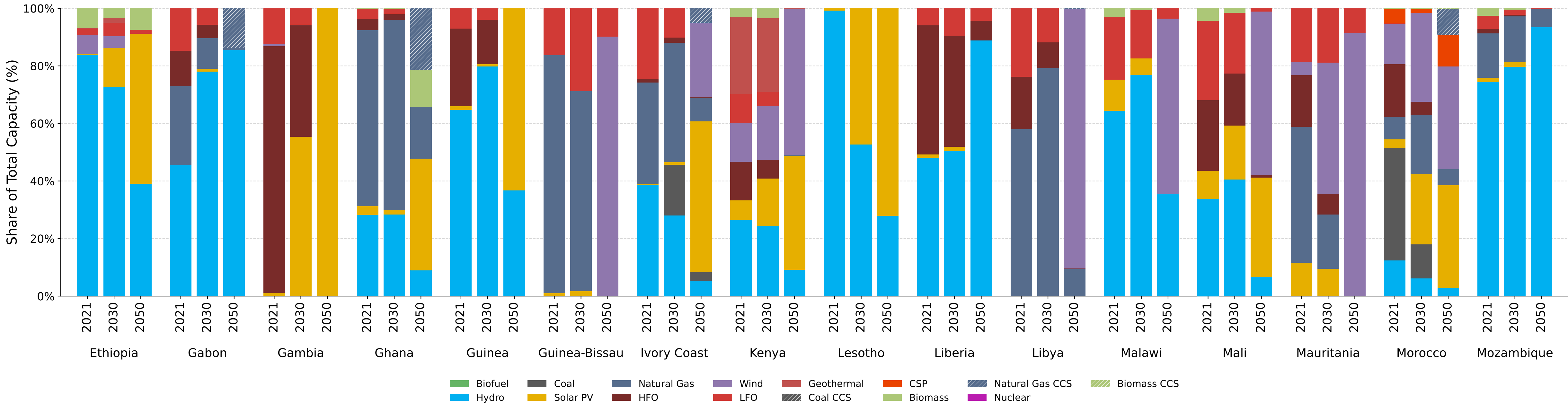
Africa – Technology Share in Installed Capacity (2021, 2030, 2050) – UNNZ
