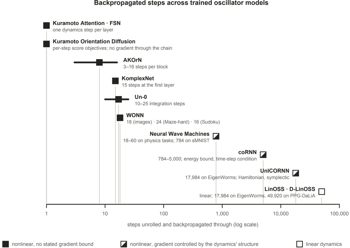
Figure 12: Steps unrolled and backpropagated through, by system. Filled markers are nonlinear dynamics with no stated gradient bound; half-filled markers are nonlinear dynamics whose gradients are controlled by the structure of the dynamics, a dissipative energy bound with a time-step condition in coRNN and Neural Wave Machines, and Hamiltonian conservation in UniCORN; the open marker is linear dynamics. Every nonlinear system without a stated bound trains at twenty-five steps or fewer; the two nonlinear systems that reach thousands of steps carry a proof, and the only system beyond twenty thousand is linear.
