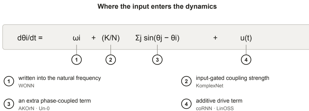
Figure 11: The four ways input enters the dynamics across the surveyed systems, each marked against the term it modifies. Classical theory makes this consequential rather than incidental: entrainment requires a phase-dependent term, so writing input into the natural frequency (1) and adding it as a drive (4) are not interchangeable. No paper in this survey contrasts two injection forms under controls.
