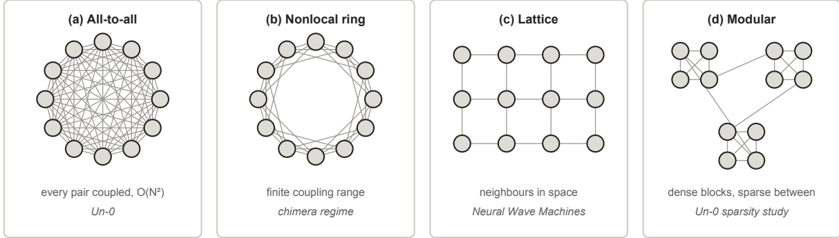
Figure 5: Four coupling geometries over the same twelve oscillators. All-to-all coupling with a free weight per pair is what Un-0 uses, and its O(N^2) parameter cost is the bulk of Un-0’s 322M parameters at 16k oscillators; AKOrN and WONN reach every pair through attention weights instead, and AKOrN’s convolutional variant couples a fixed neighbourhood. Finite coupling range is the case the physics canon reports chimera states in. A lattice is the geometry of Neural Wave Machines. The modular fabric is the best performer in the one published sparsity study of a trained oscillator network, which is blog-published and covers one system.
