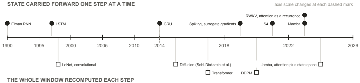
Figure 8: Conventional neural network architectures, by how each one holds the past. Above the axis, a state is carried forward one step at a time; below it, the whole window is recomputed at every step. Diffusion sits below the axis as well: it keeps nothing between inputs and iterates a denoiser over noise levels rather than over time, the iteration Kuramoto Orientation Diffusion makes oscillatory. An oscillator field belongs to the upper track, but its state evolves under a fixed differential equation rather than under a transition learned from scratch, which is the substance of both the efficiency argument made for it and the training difficulty reported against it.
