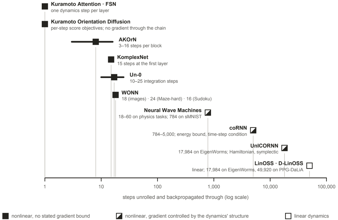
Figure 12: Steps unrolled and backpropagated through, by system. Filled markers are nonlinear dynamics with no stated gradient bound; half-filled markers are nonlinear dynamics whose gradients are controlled by the structure of the dynamics, a dissipative energy bound with a time-step condition in coRNN and Neural Wave Machines, and Hamiltonian conservation in UnICORNN; the open marker is linear dynamics. Every nonlinear system without a stated bound trains at twenty-five steps or fewer; the two nonlinear systems that reach thousands of steps carry a proof, and the only system beyond twenty thousand is linear.
