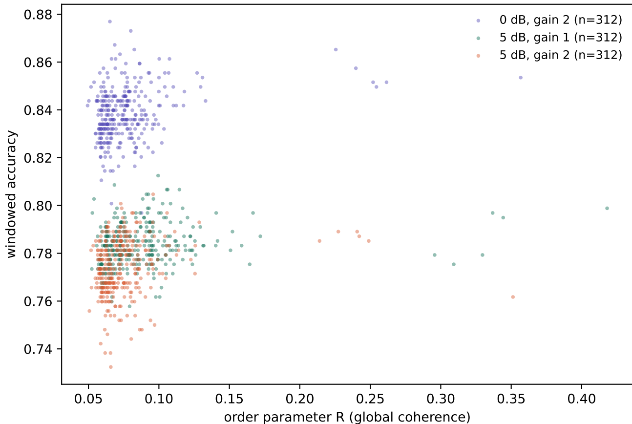
Untrained runs: readability vs coherence
