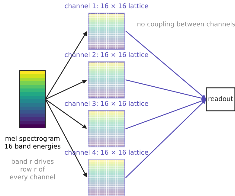
(b) Channels: side by side, all driven by the same input (width)
