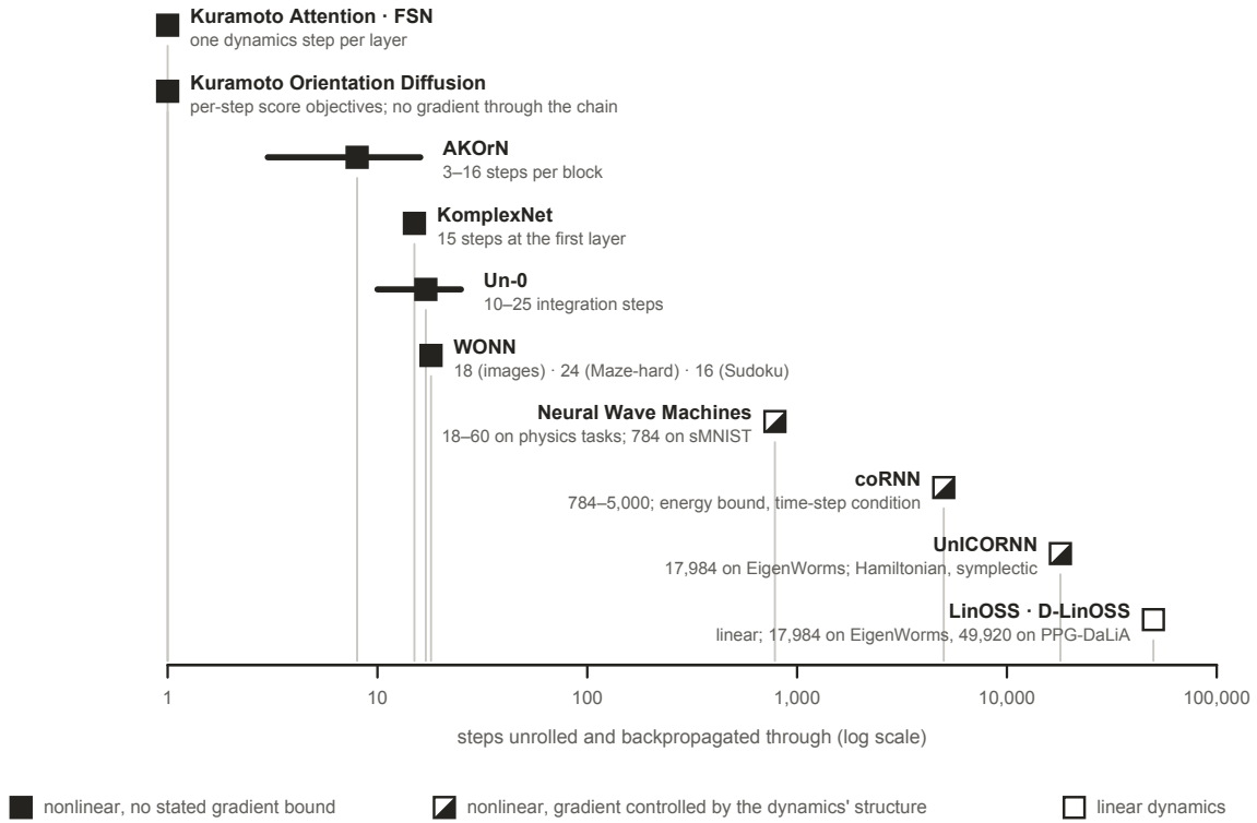
Figure 12: Steps unrolled and backpropagated through, by system. Filled markers are nonlinear dynamics with no stated gradient bound; half-filled markers are nonlinear dynamics whose gradients are controlled by the structure of the dynamics, a dissipative energy bound with a time-step condition in coRNN and Neural Wave Machines, and Hamiltonian conservation in UniCORNN; the open marker is linear dynamics. Every nonlinear system without a stated bound trains at twenty-five steps or fewer; the two nonlinear systems that reach thousands of steps carry a proof, and the only system beyond twenty thousand is linear.
