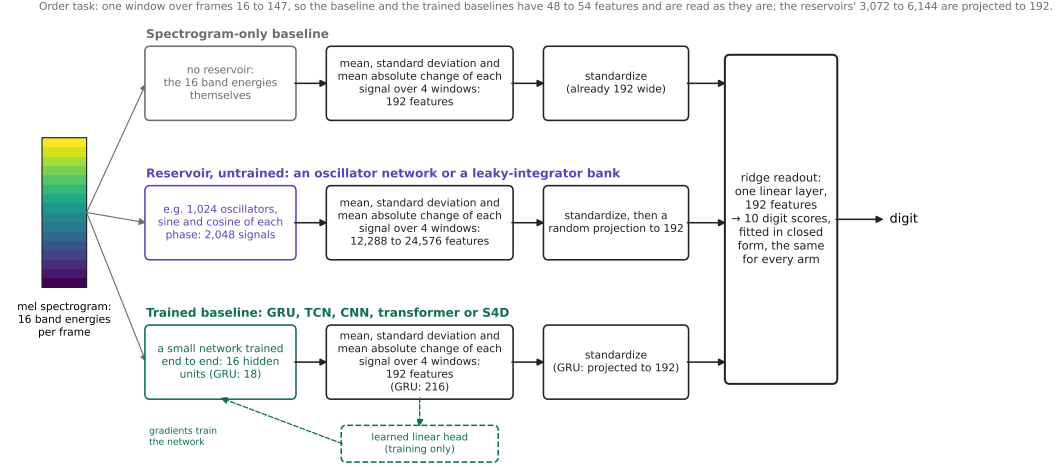
Figure 10: The read for each kind of arm: the same three statistics over the same four windows, classified by a ridge readout fitted to each arm. The spectrogram-only baseline’s 192 features are read as they are; a reservoir’s 12,288 to 24,576 are standardized and projected to 192 by a fixed random matrix; a trained baseline’s 192 (the GRU’s 216, projected) are read after the network is trained end to end through a learned linear head.
