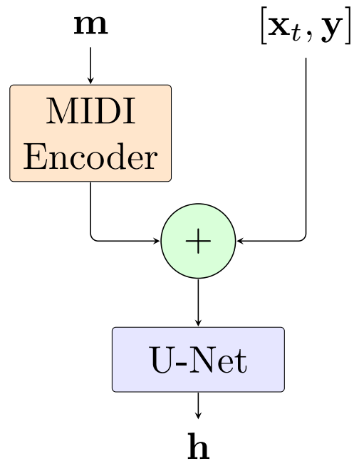
Early Injection
