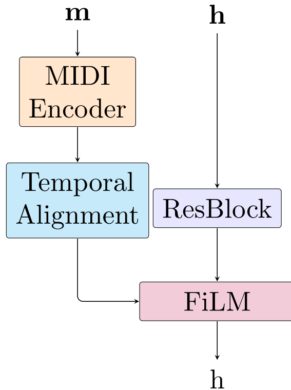
FiLM
