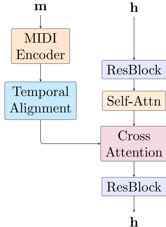
Cross-Attention
