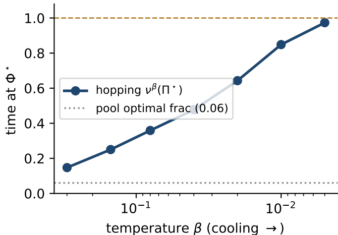
Hopping concentrates on the optimum
