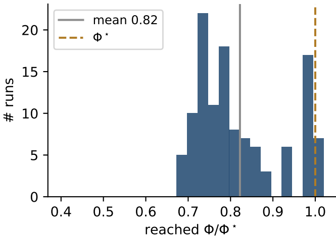
Independent learning traps ( k=5 )
