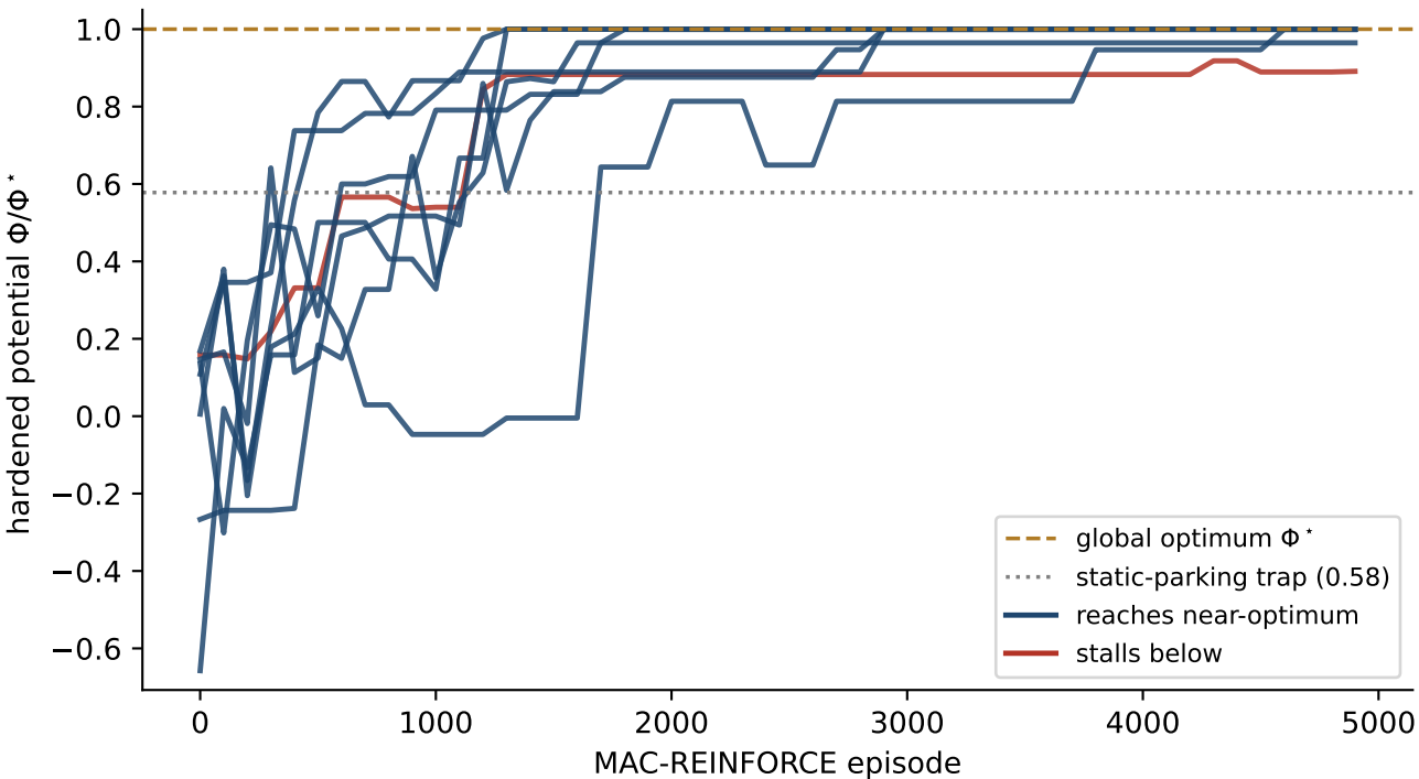
Drone game: blind coordination ascends the shared potential ( n=3 , H=1 ) independent per-agent learning, no communication
