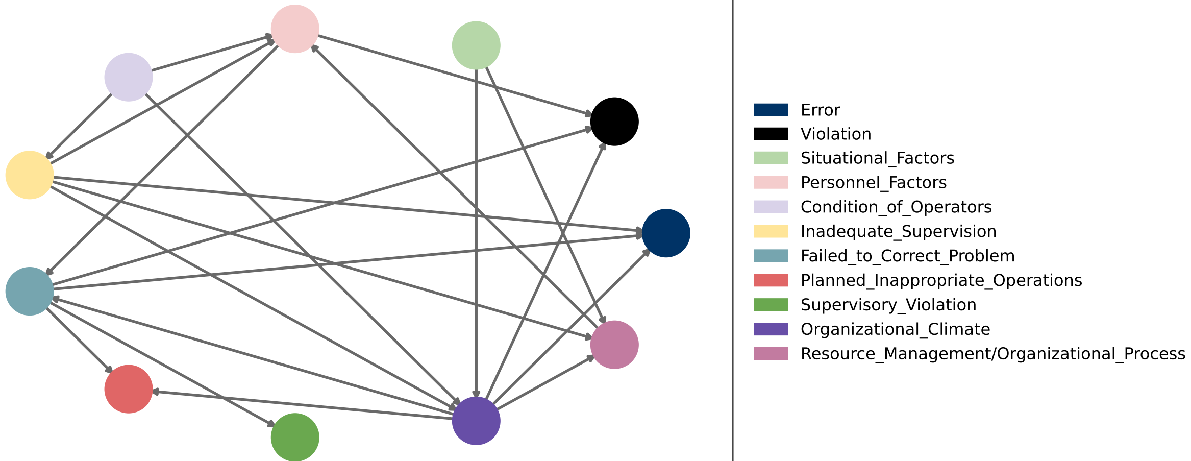
Learned HFACS DAG (GES optimized)
