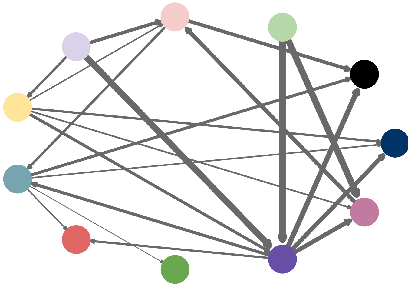
Learned HFACS DAG (GES optimized)
