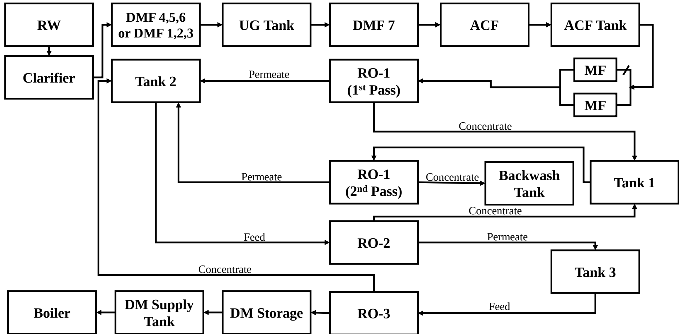
Figure: KPCL WTP Flow Diagram.
