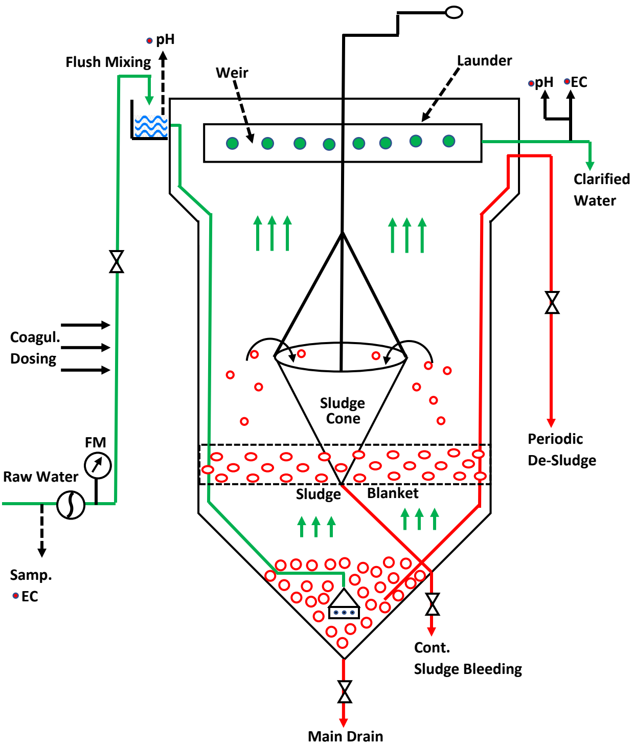
Fig: VERTICAL FLOW CLARIFIER
