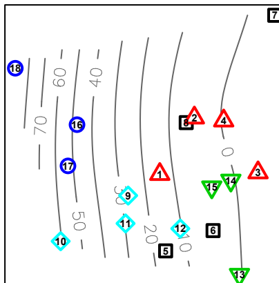
Square root transformed
