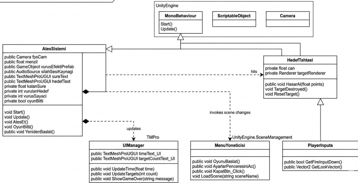
DUNE HUNTER - GAME CLASS DIAGRAM (UML)
