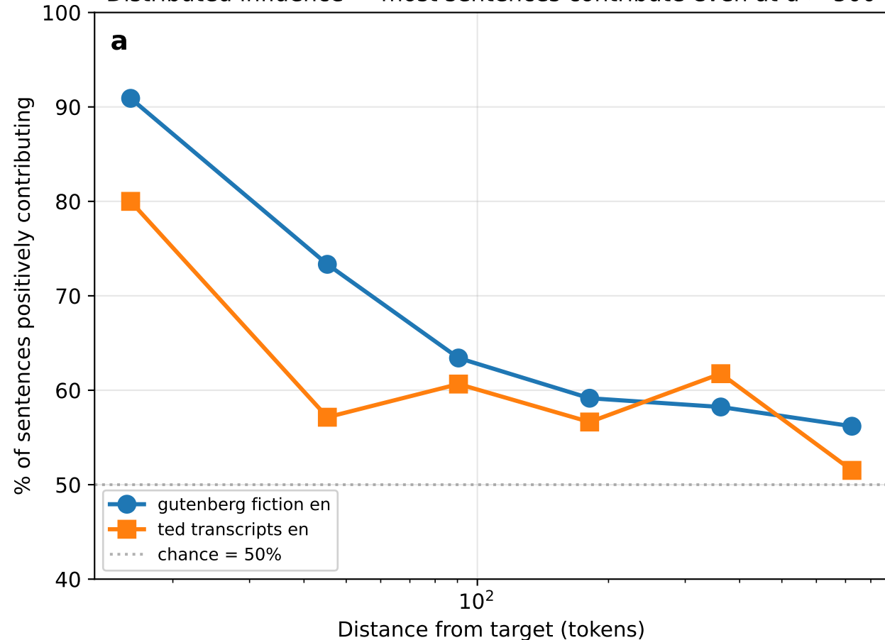
Distributed influence — most sentences contribute even at d > 500
