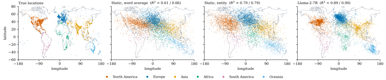
Figure 1: Held-out places from Gurnee and Tegmark (2024) that have a Wikipedia2Vec entity vector ( n = 5,984 ), at their true locations and as decoded by linear probes on Wikipedia2Vec’s word vectors averaged over the name, on its static entity vectors, and on Llama-2-7B (layer 24), drawn over coastlines as in Gurnee and Tegmark (2024)’s Figure 1 (which shows Llama-2-70B); color marks the true continent. The entity vectors recover a blurred version of the layout that Llama-2 recovers more precisely (median error 2,450 km against 760 km; Table 2).
