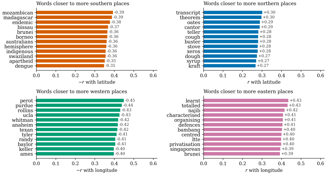
Figure 2: Words whose GloVe vectors are most similar to place names that lie farther south, north, west or east. For each of 15,923 words (the 20,000 most frequent GloVe words with at least four letters, excluding a list of country names, demonyms and geographic terms and any word that is part of at least three place names), we correlate the word’s cosine similarity to the averaged name vector of each of the 33,500 released places that have a GloVe vector with the place’s latitude or longitude; shown are the twelve strongest correlations at each end. The words are selected for extreme correlations from the whole vocabulary, so the figure is descriptive and implies no significance.
