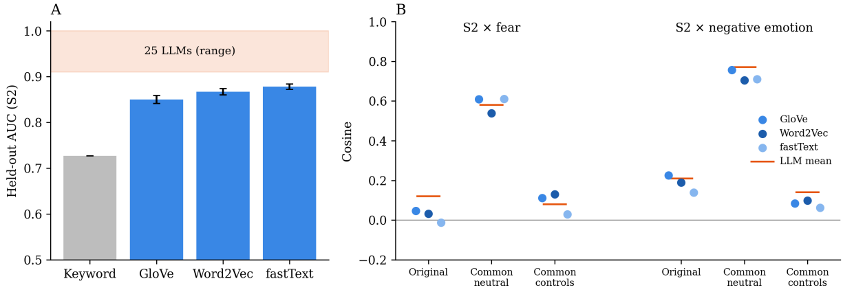
Figure 3: The representational tests reported for a “pain axis” in 25 LLMs (Tagliabue et al., 2026), run on averaged static word vectors of the authors’ own sentences. A : held-out separation of pain from controls (S2, first person; five-fold cross-validation over sentence sets, mean \pm s.d. over 20 fold assignments). The keyword baseline is the best of several surface-lexical classifiers reported by an independent review (pain-axis-review contributors, 2026). LLM values are each model’s best layer. B : cosine of the pain direction with fear, negative-emotion and negative-world-state directions; bars span the LLMs’ per-model range.
