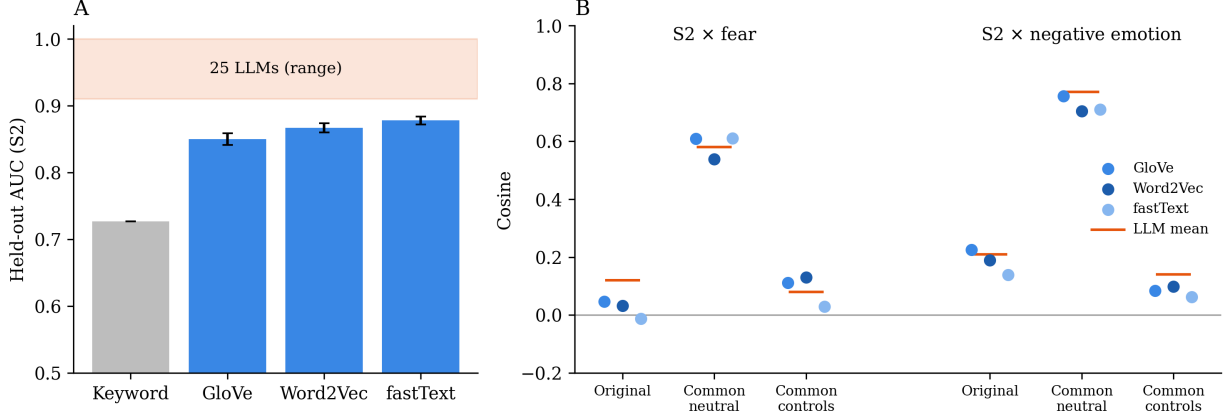
Figure 3: The representational tests reported for a “pain axis” in 25 LLMs (Tagliabue et al., 2026), run on averaged static word vectors of the authors’ own sentences. A : held-out separation of pain from controls (S2, first person; five-fold cross-validation over sentence sets, mean \pm s.d. over 20 fold assignments). The keyword baseline is the best of several surface-lexical classifiers reported by an independent review (pain-axis-review contributors, 2026). LLM values are each model’s best layer. B : cosine of the pain direction with fear, negative-emotion and negative-world-state directions; bars span the LLMs’ per-model range.
