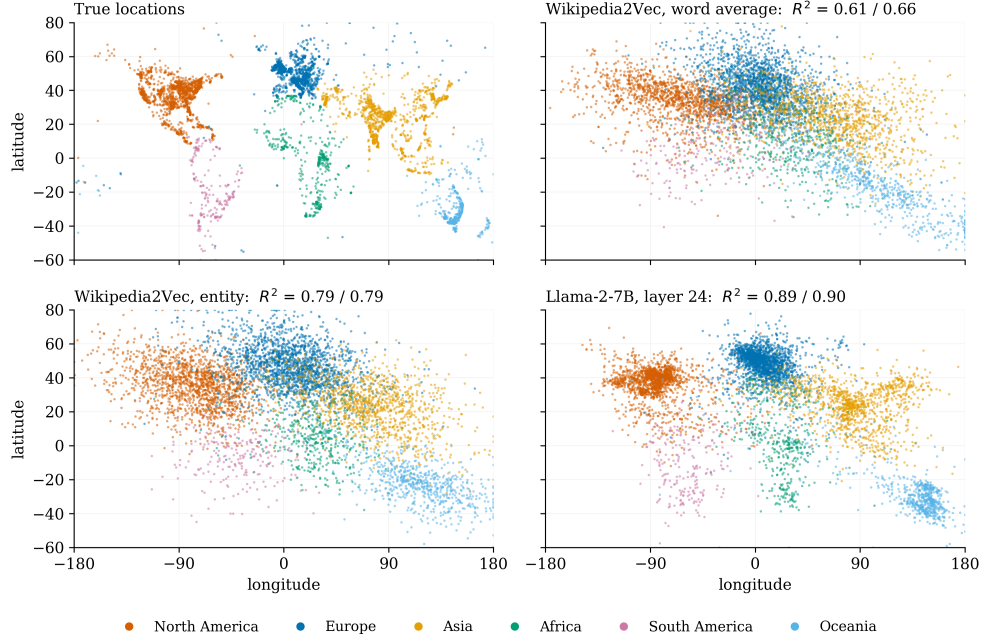
Figure 1: Held-out places from Gurnee and Tegmark (2024) that have a Wikipedia2Vec entity vector ( n = 5,984 ), at their true locations and as decoded by linear probes on Wikipedia2Vec’s word vectors averaged over the name, on its static entity vectors, and on Llama-2-7B (layer 24), as in Gurnee and Tegmark (2024)’s Figure 1 (which shows Llama-2-70B); color marks the true continent. Panel titles give R^2 for latitude / longitude over all places; four places in Antarctica are not drawn. The entity vectors recover a blurred version of the layout that Llama-2 recovers more precisely (median error 2,450 km against 760 km; Table 2).
