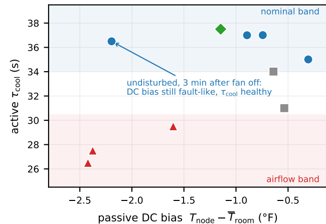
(c) Passive DC bias vs. active time constant
