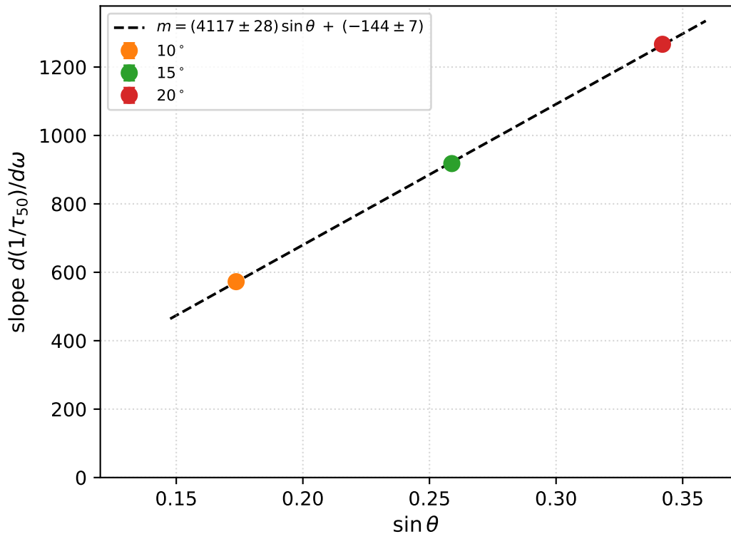
Angle dependence of the \omega -scaling slope
