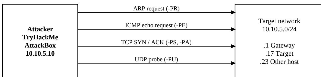
Fig 2: Working of a host discovery scan
