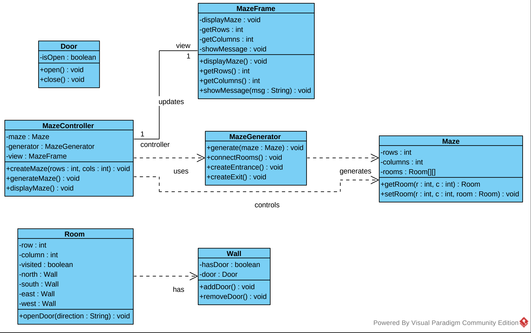
Maze Generation System Class Diagram
