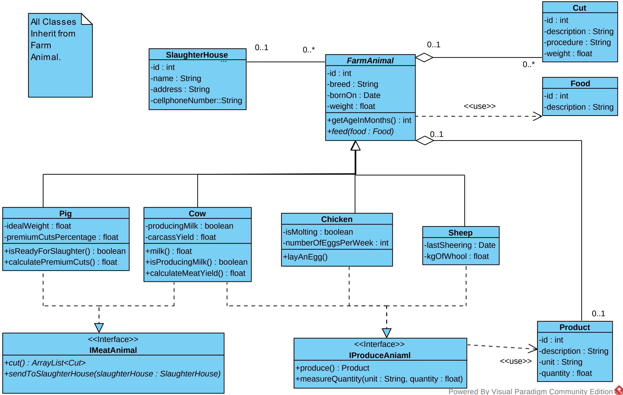
Class Diagram1
