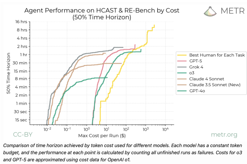
Figure 16: Agent Performance on HCAST & RE-Bench by Cost
